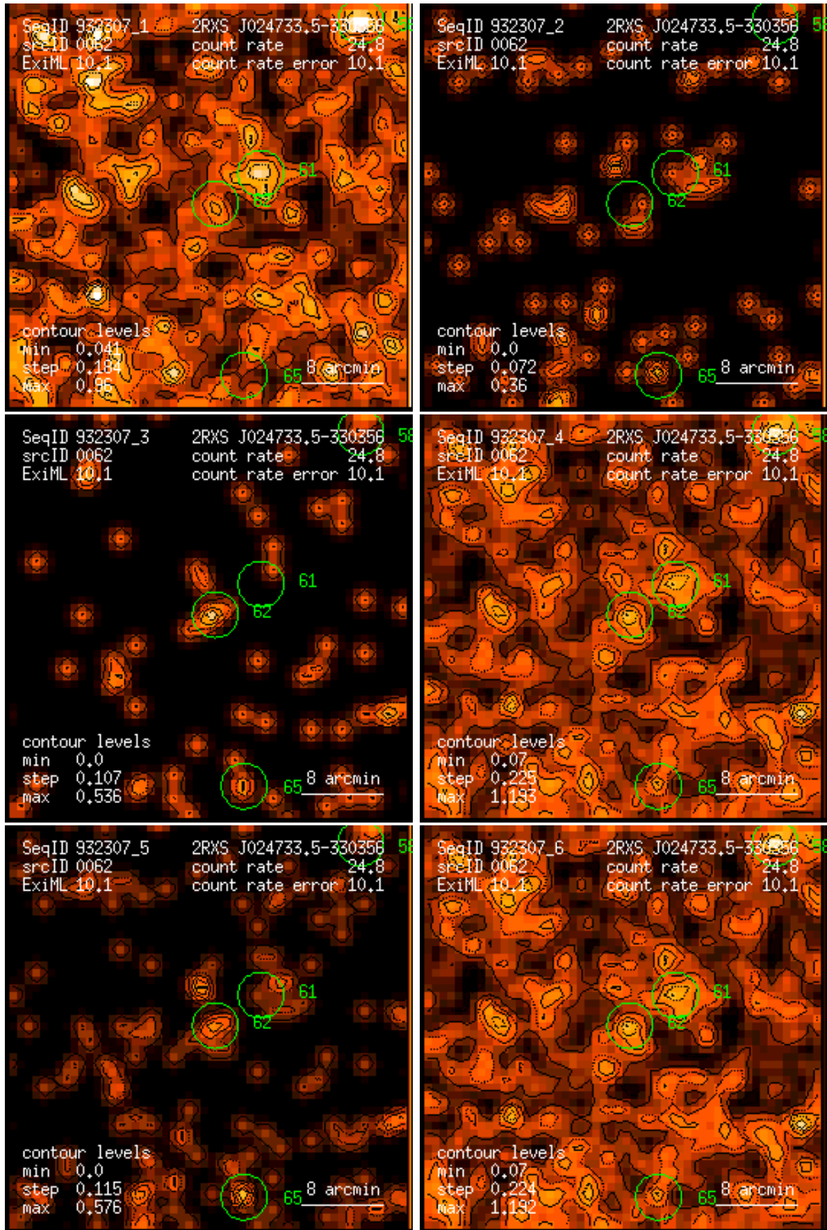
Figure 62: RASS 932307: detection 0062: band rate images, Gaussian filter: (1) PSPC channels 11 – 41, (2) 52 – 90, (3) 91 – 201, (4) 11 – 235, (5) 52 – 201, (6) 11 – 201. Broad band rates in counts/ks. Band rate contour levels in counts/ks/arcmin 2 .
