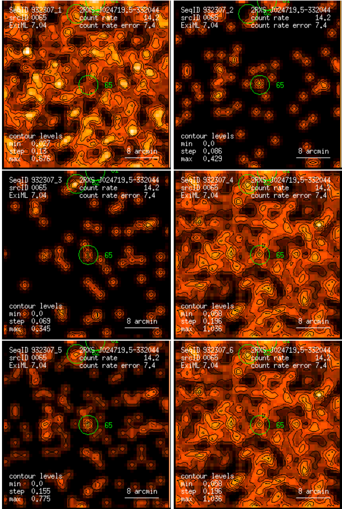
Figure 65: RASS 932307: detection 0065: band rate images, Gaussian filter: (1) PSPC channels 11 – 41, (2) 52 – 90, (3) 91 – 201, (4) 11 – 235, (5) 52 – 201, (6) 11 – 201. Broad band rates in counts/ks. Band rate contour levels in counts/ks/arcmin 2 .
