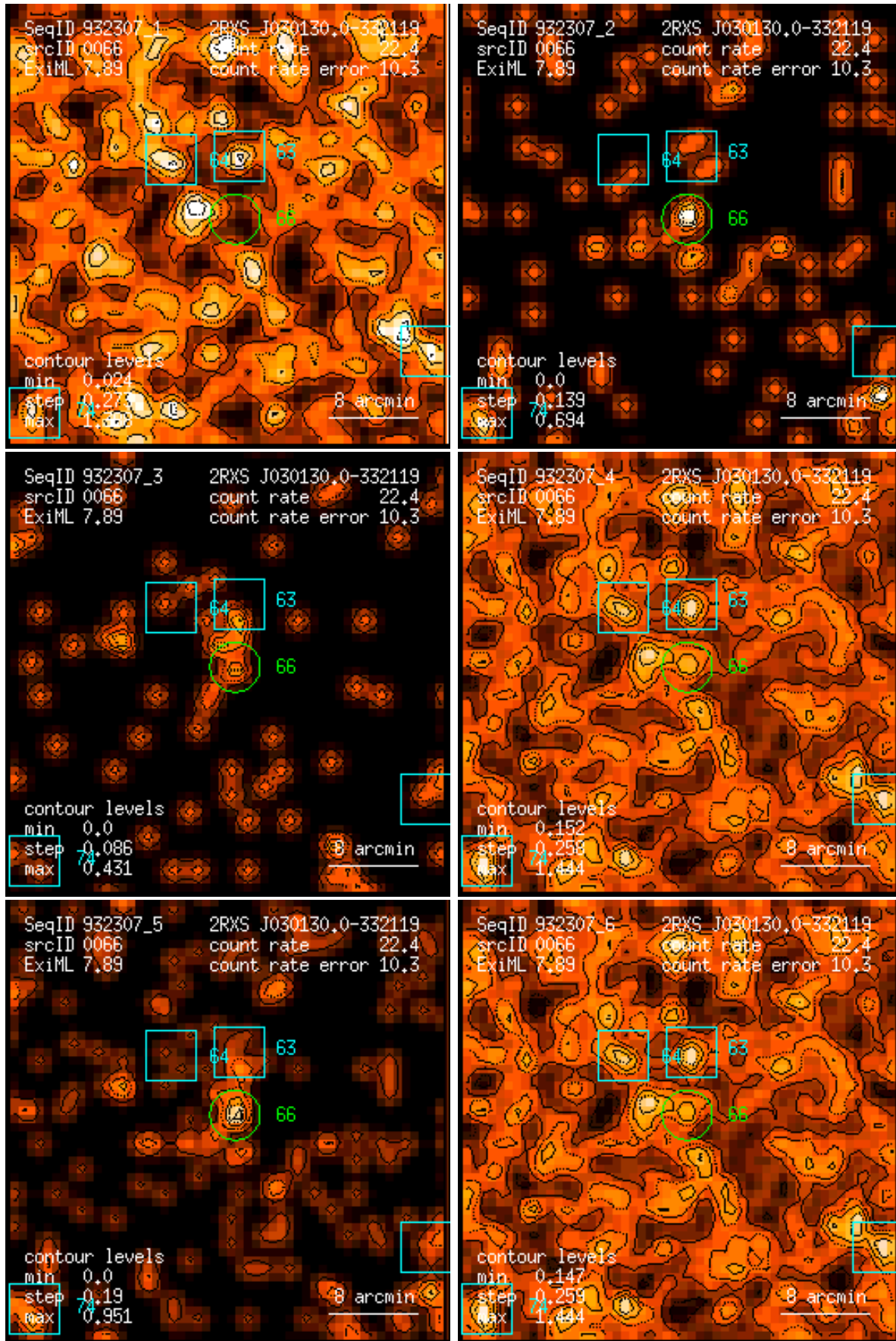
Figure 66: RASS 932307: detection 0066: band rate images, Gaussian filter: (1) PSPC channels 11 – 41, (2) 52 – 90, (3) 91 – 201, (4) 11 – 235, (5) 52 – 201, (6) 11 – 201. Broad band rates in counts/ks. Band rate contour levels in counts/ks/arcmin 2 .
