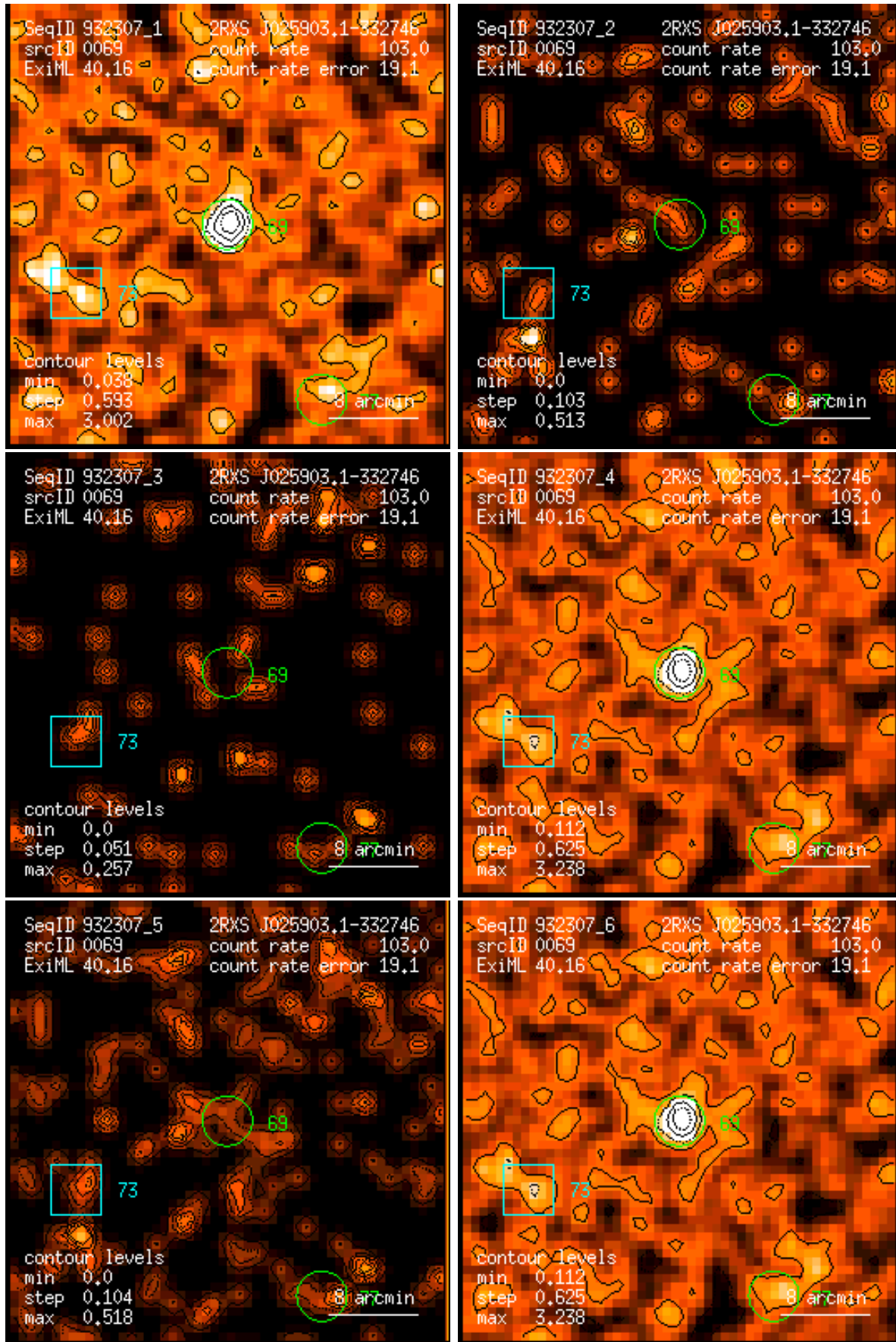
Figure 69: RASS 932307: detection 0069: band rate images, Gaussian filter: (1) PSPC channels 11 – 41, (2) 52 – 90, (3) 91 – 201, (4) 11 – 235, (5) 52 – 201, (6) 11 – 201. Broad band rates in counts/ks. Band rate contour levels in counts/ks/arcmin 2 .
