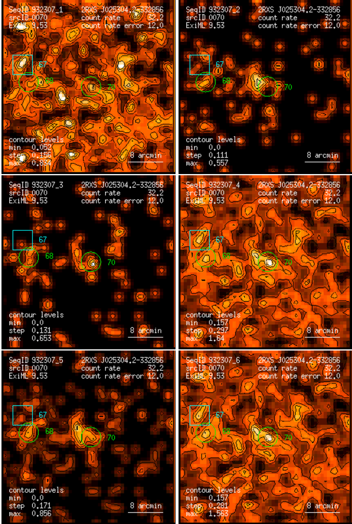
Figure 70: RASS 932307: detection 0070: band rate images, Gaussian filter: (1) PSPC channels 11 – 41, (2) 52 – 90, (3) 91 – 201, (4) 11 – 235, (5) 52 – 201, (6) 11 – 201. Broad band rates in counts/ks. Band rate contour levels in counts/ks/arcmin 2 .
