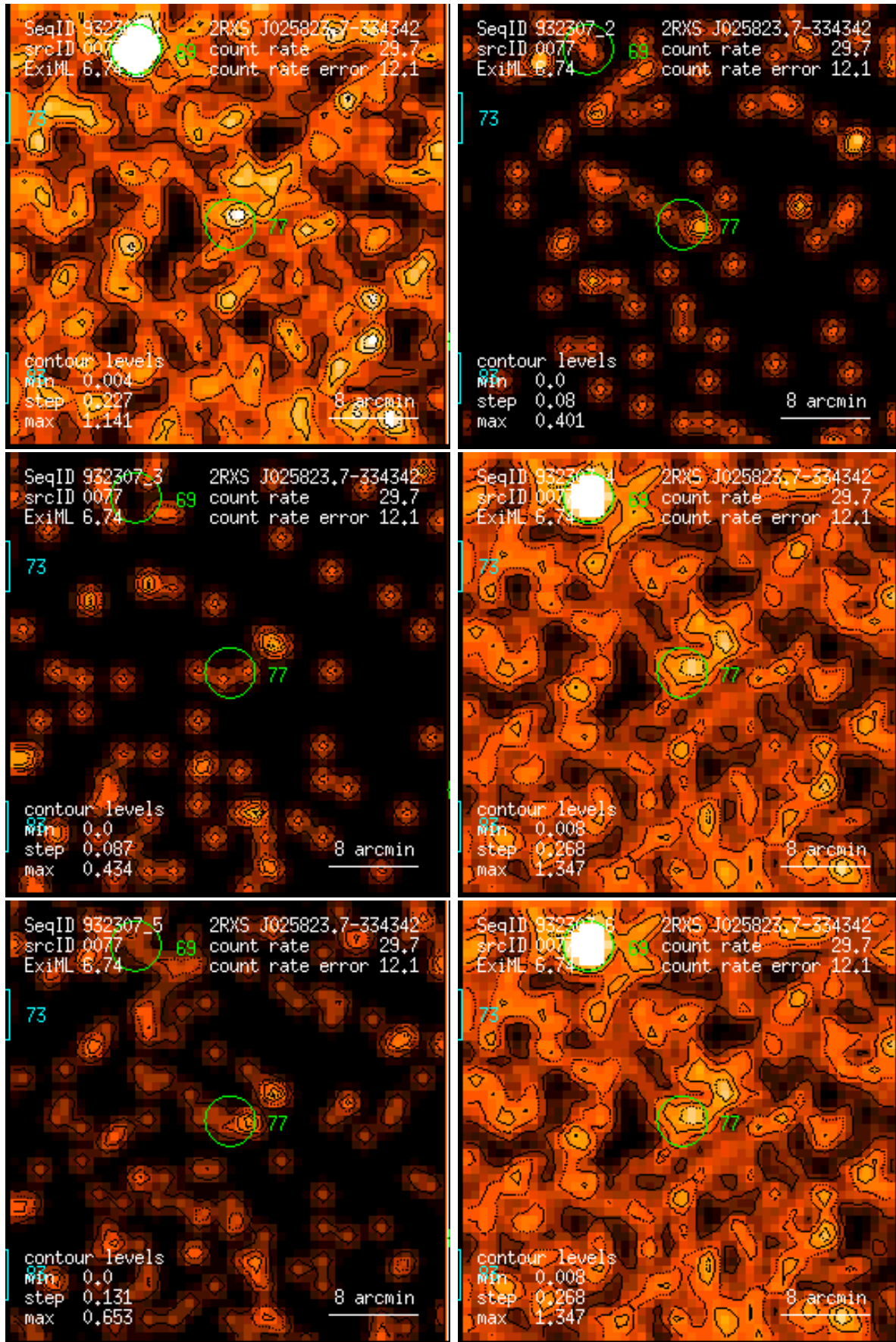
Figure 77: RASS 932307: detection 0077: band rate images, Gaussian filter: (1) PSPC channels 11 – 41, (2) 52 – 90, (3) 91 – 201, (4) 11 – 235, (5) 52 – 201, (6) 11 – 201. Broad band rates in counts/ks. Band rate contour levels in counts/ks/arcmin 2 .
