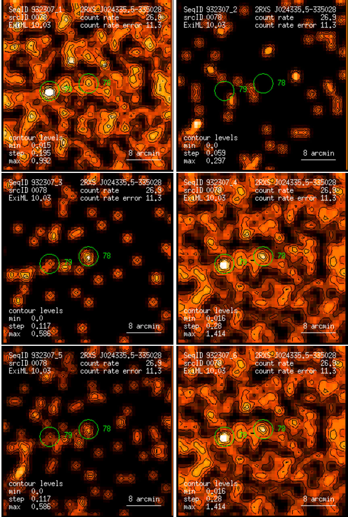
Figure 78: RASS 932307: detection 0078: band rate images, Gaussian filter: (1) PSPC channels 11 – 41, (2) 52 – 90, (3) 91 – 201, (4) 11 – 235, (5) 52 – 201, (6) 11 – 201. Broad band rates in counts/ks. Band rate contour levels in counts/ks/arcmin 2 .
