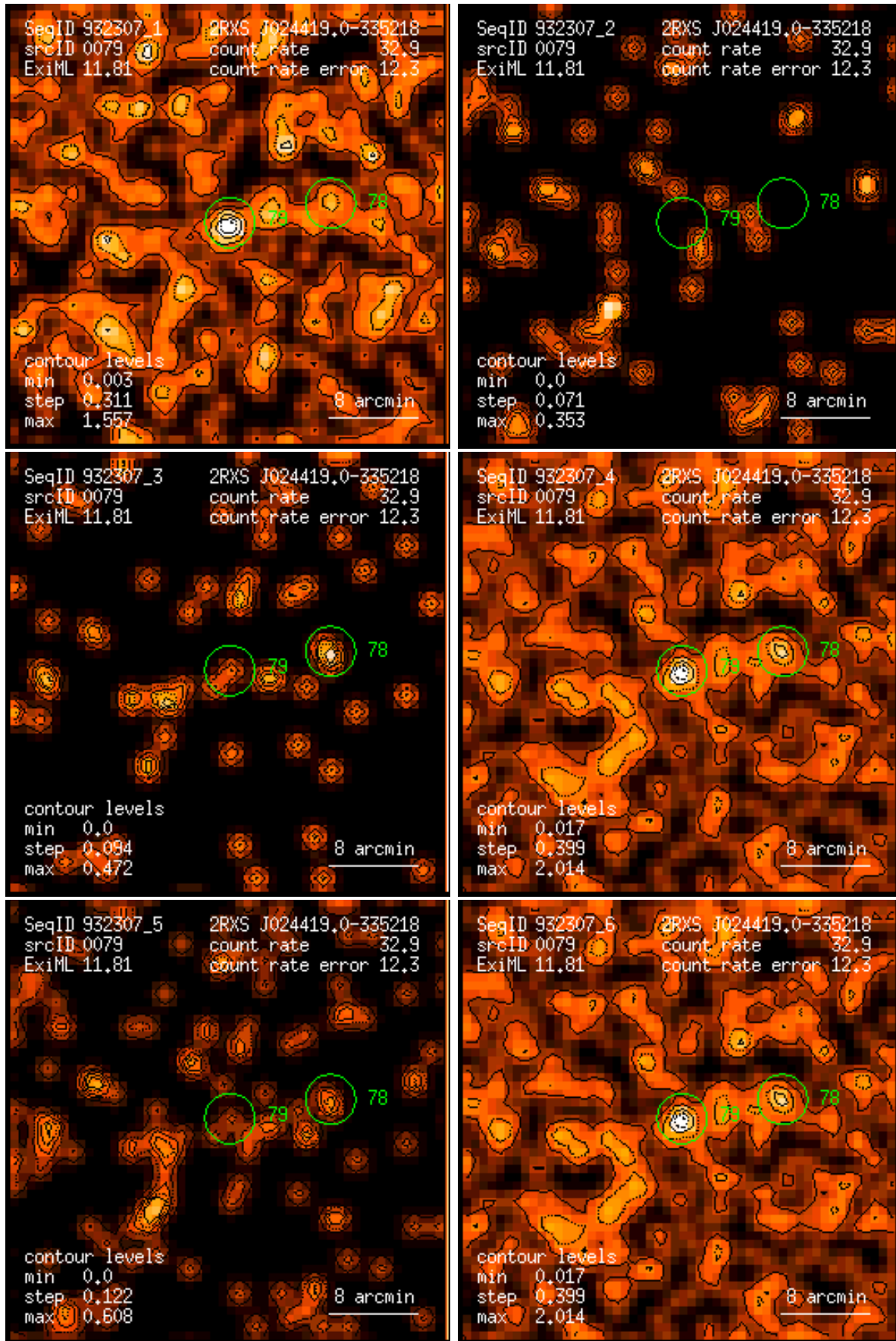
Figure 79: RASS 932307: detection 0079: band rate images, Gaussian filter: (1) PSPC channels 11 – 41, (2) 52 – 90, (3) 91 – 201, (4) 11 – 235, (5) 52 – 201, (6) 11 – 201. Broad band rates in counts/ks. Band rate contour levels in counts/ks/arcmin 2 .
