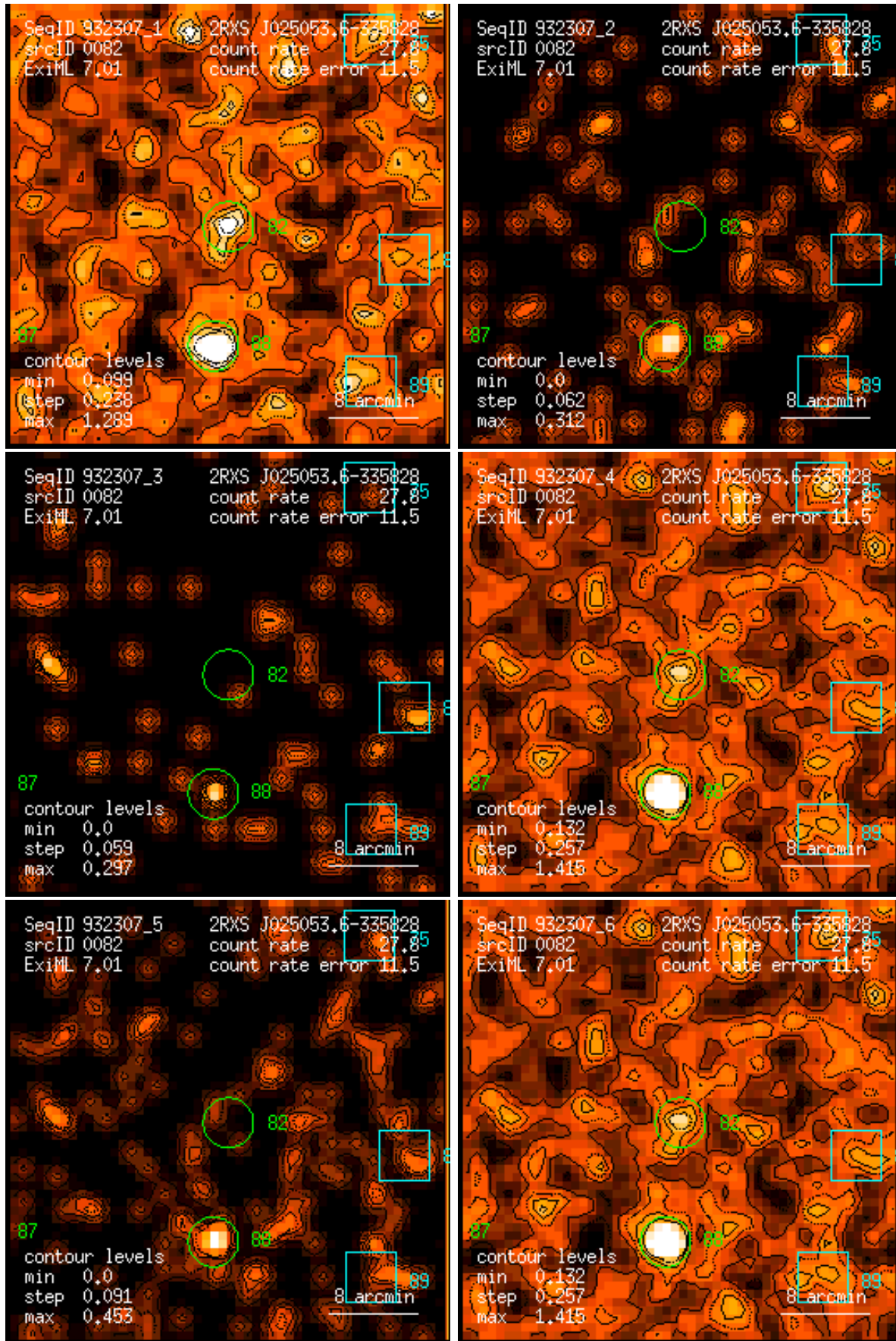
Figure 82: RASS 932307: detection 0082: band rate images, Gaussian filter: (1) PSPC channels 11 – 41, (2) 52 – 90, (3) 91 – 201, (4) 11 – 235, (5) 52 – 201, (6) 11 – 201. Broad band rates in counts/ks. Band rate contour levels in counts/ks/arcmin 2 .
