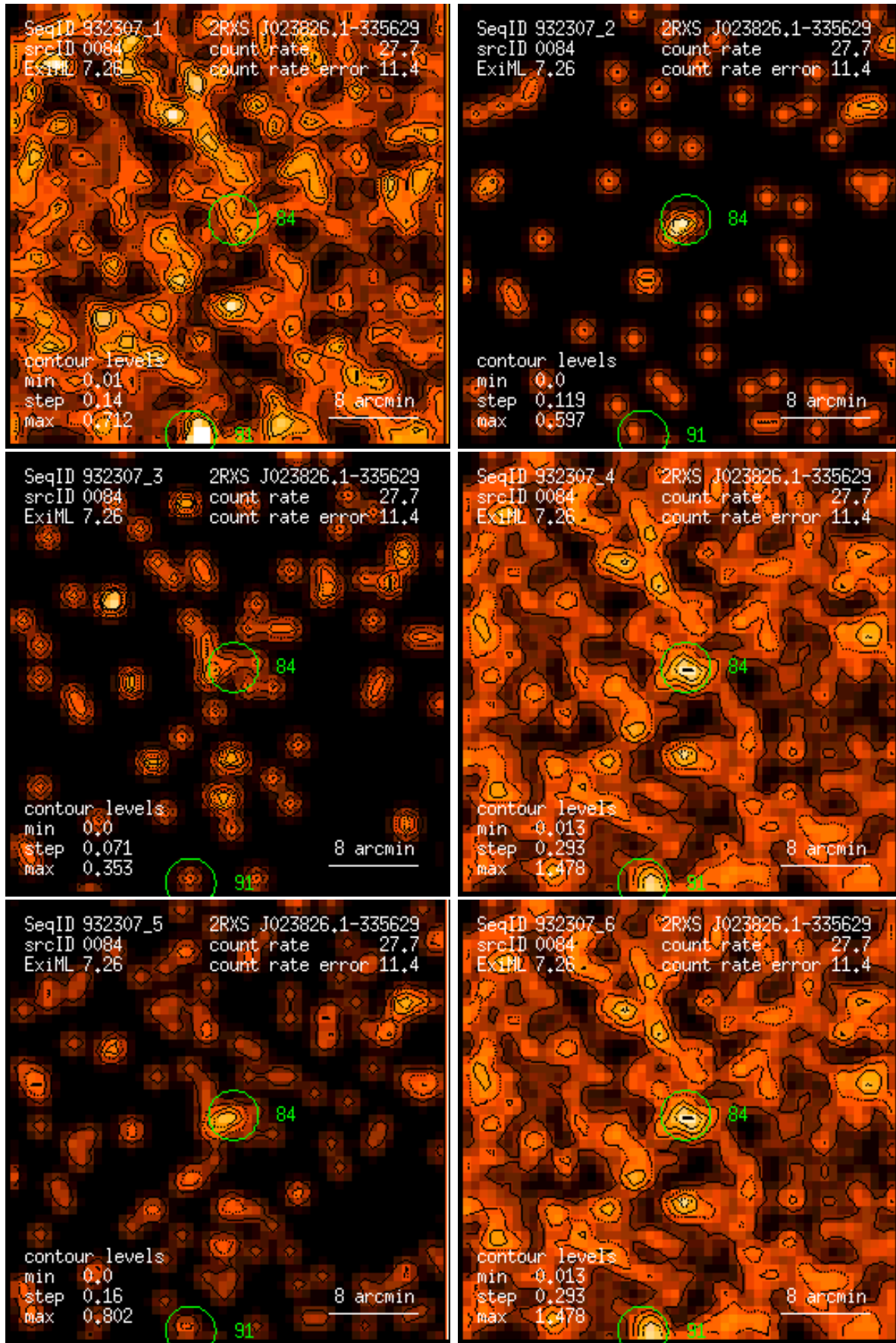
Figure 84: RASS 932307: detection 0084: band rate images, Gaussian filter: (1) PSPC channels 11 – 41, (2) 52 – 90, (3) 91 – 201, (4) 11 – 235, (5) 52 – 201, (6) 11 – 201. Broad band rates in counts/ks. Band rate contour levels in counts/ks/arcmin 2 .
