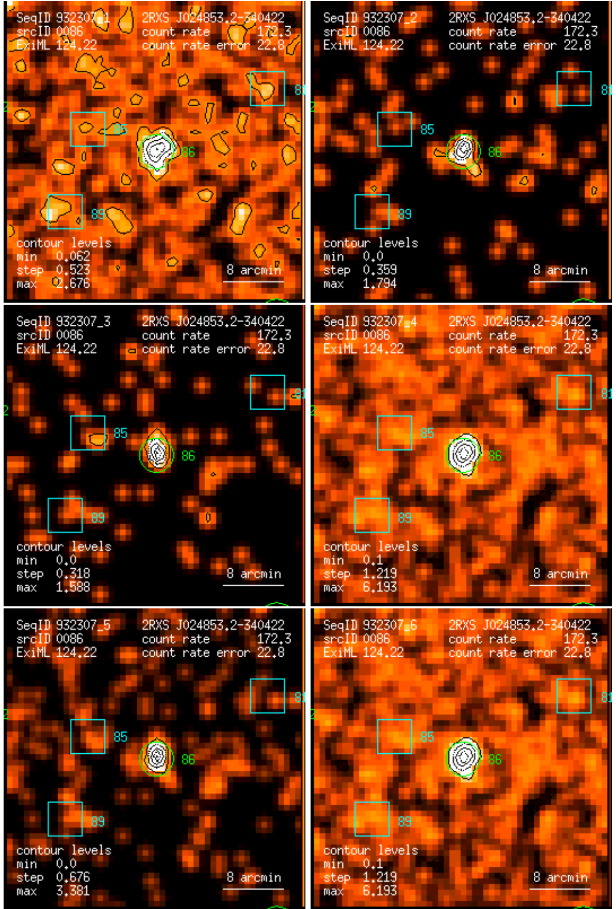
Figure 86: RASS 932307: detection 0086: band rate images, Gaussian filter: (1) PSPC channels 11 – 41, (2) 52 – 90, (3) 91 – 201, (4) 11 – 235, (5) 52 – 201, (6) 11 – 201. Broad band rates in counts/ks. Band rate contour levels in counts/ks/arcmin 2 .
