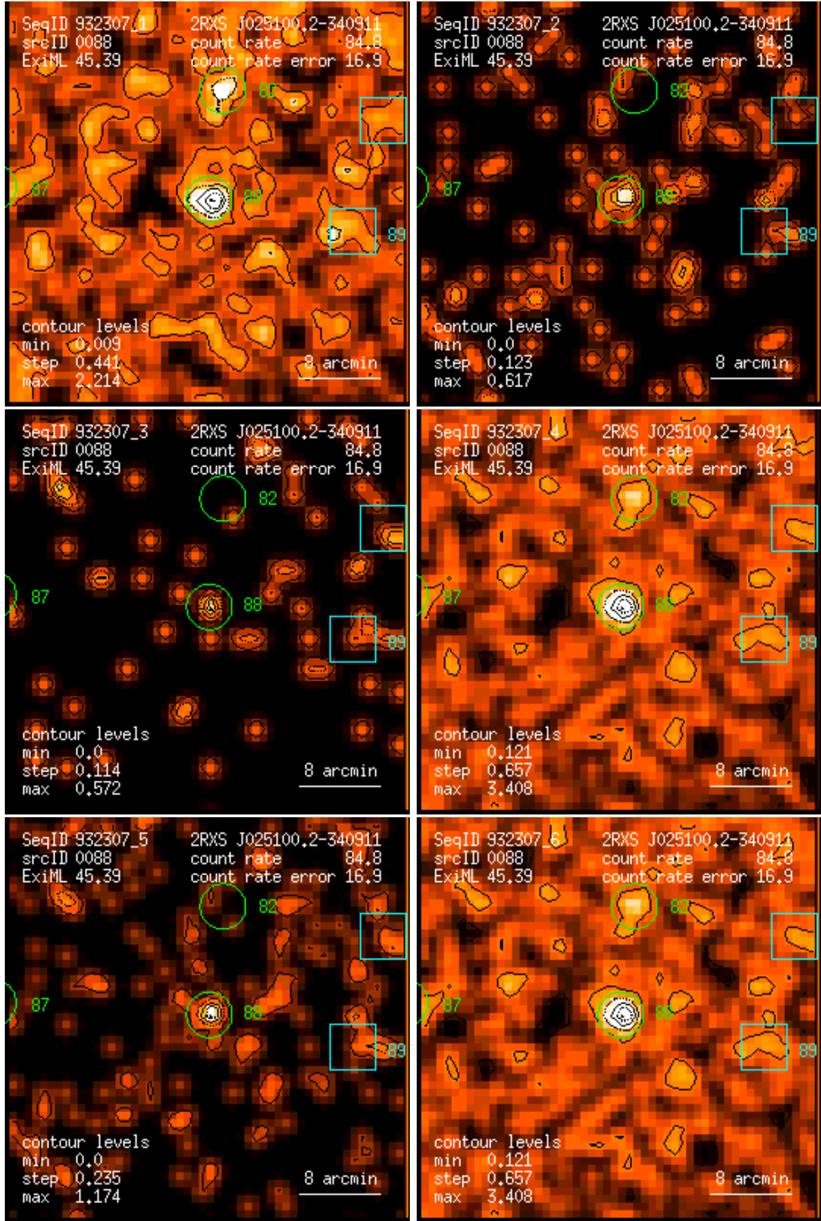
Figure 88: RASS 932307: detection 0088: band rate images, Gaussian filter: (1) PSPC channels 11 – 41, (2) 52 – 90, (3) 91 – 201, (4) 11 – 235, (5) 52 – 201, (6) 11 – 201. Broad band rates in counts/ks. Band rate contour levels in counts/ks/arcmin 2 .
