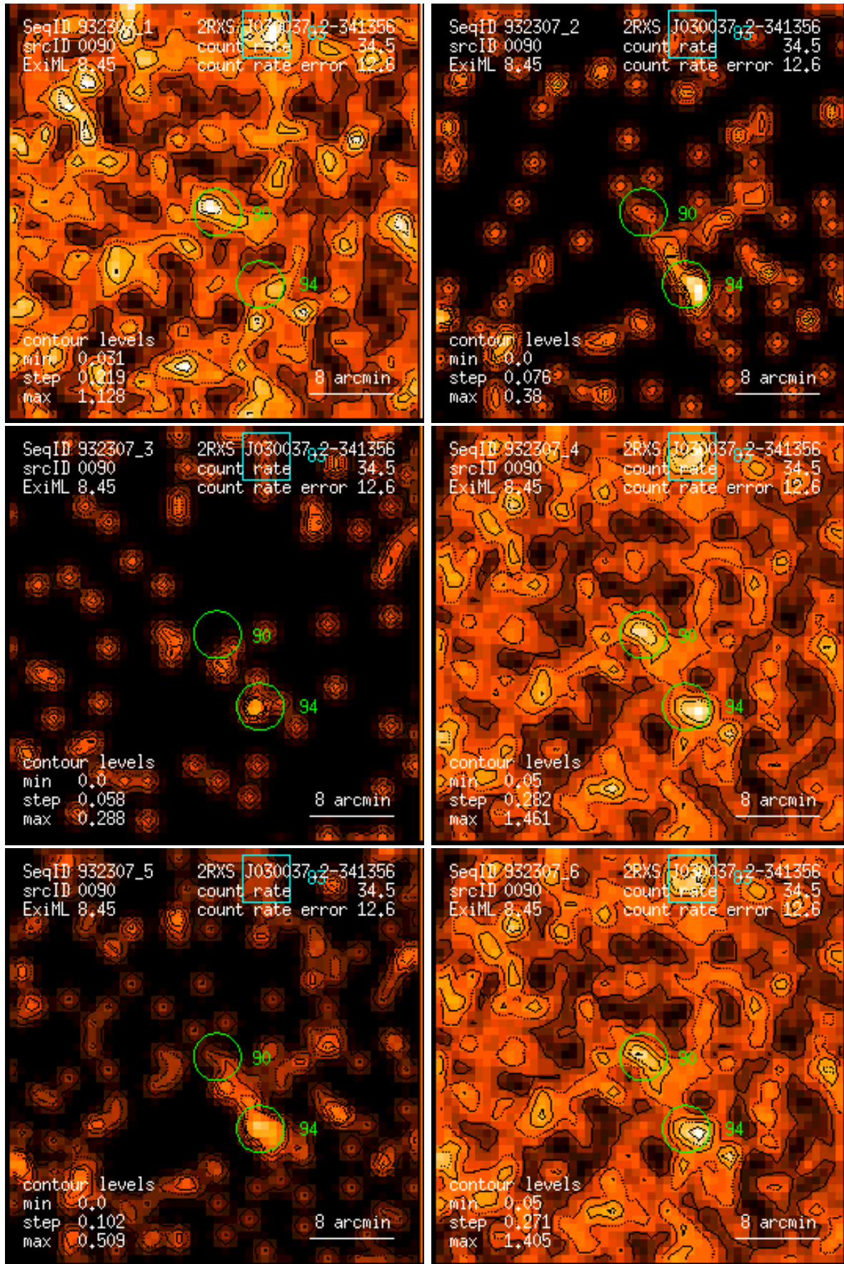
Figure 90: RASS 932307: detection 0090: band rate images, Gaussian filter: (1) PSPC channels 11 – 41, (2) 52 – 90, (3) 91 – 201, (4) 11 – 235, (5) 52 – 201, (6) 11 – 201. Broad band rates in counts/ks. Band rate contour levels in counts/ks/arcmin 2 .
