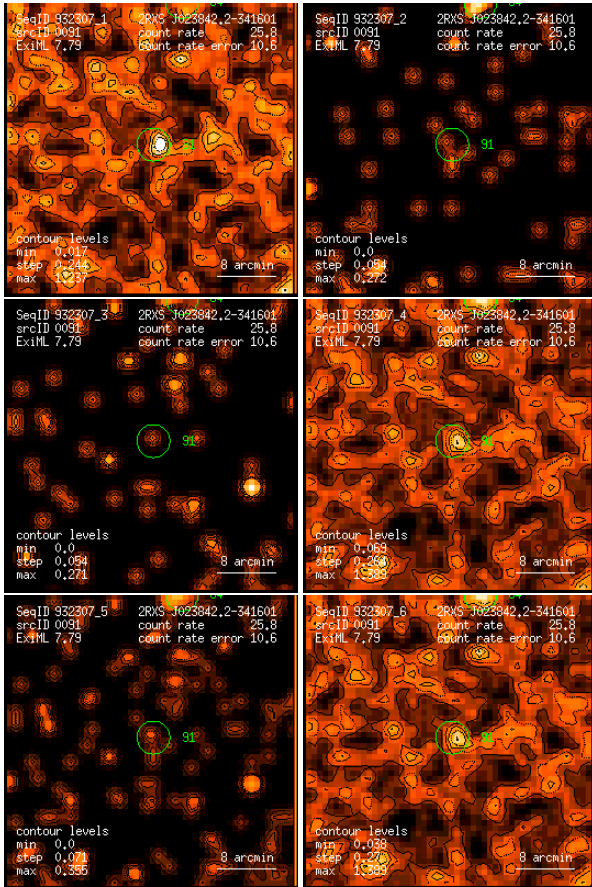
Figure 91: RASS 932307: detection 0091: band rate images, Gaussian filter: (1) PSPC channels 11 – 41, (2) 52 – 90, (3) 91 – 201, (4) 11 – 235, (5) 52 – 201, (6) 11 – 201. Broad band rates in counts/ks. Band rate contour levels in counts/ks/arcmin 2 .
