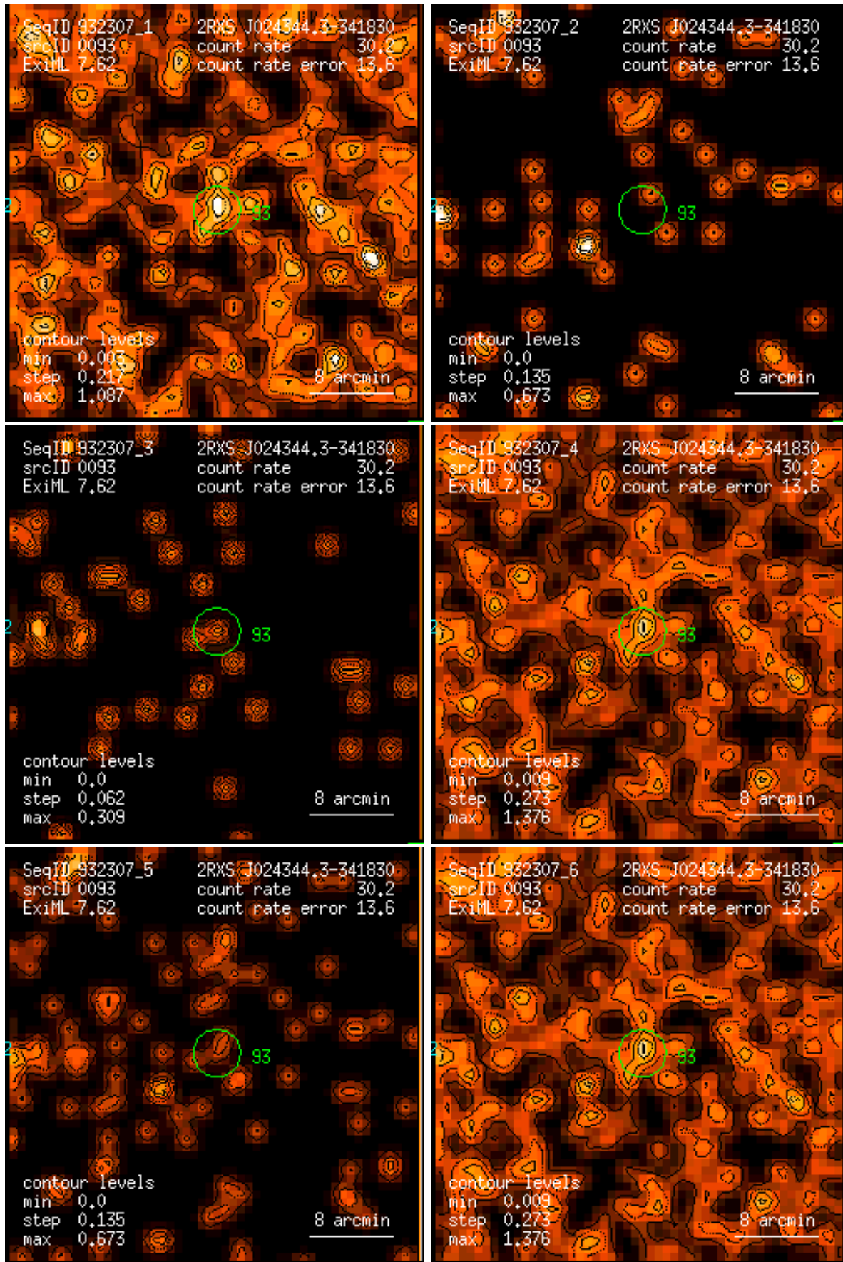
Figure 93: RASS 932307: detection 0093: band rate images, Gaussian filter: (1) PSPC channels 11 – 41, (2) 52 – 90, (3) 91 – 201, (4) 11 – 235, (5) 52 – 201, (6) 11 – 201. Broad band rates in counts/ks. Band rate contour levels in counts/ks/arcmin 2 .
