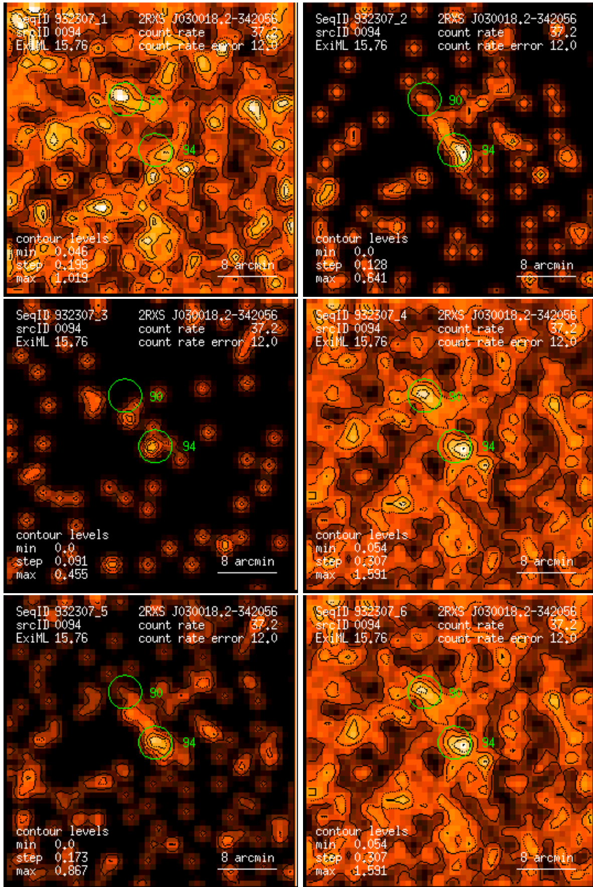
Figure 94: RASS 932307: detection 0094: band rate images, Gaussian filter: (1) PSPC channels 11 – 41, (2) 52 – 90, (3) 91 – 201, (4) 11 – 235, (5) 52 – 201, (6) 11 – 201. Broad band rates in counts/ks. Band rate contour levels in counts/ks/arcmin 2 .
