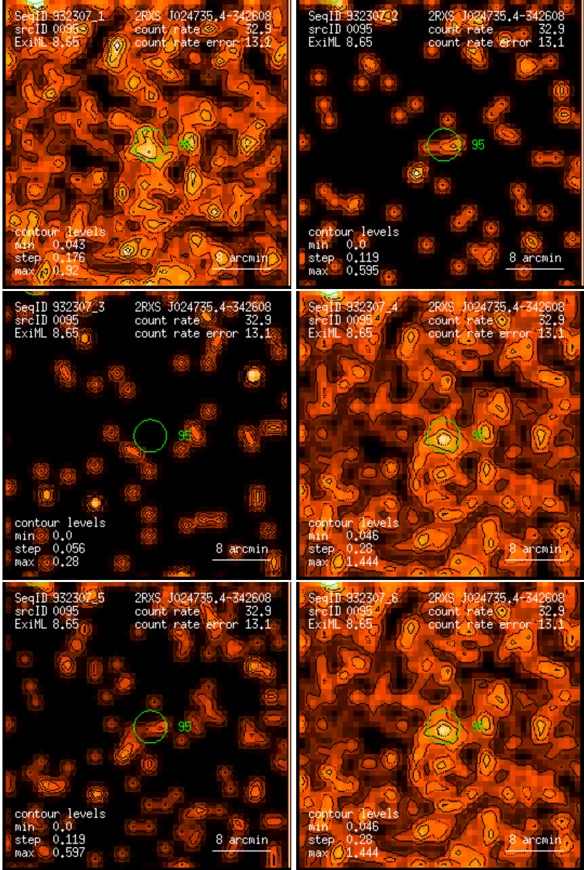
Figure 95: RASS 932307: detection 0095: band rate images, Gaussian filter: (1) PSPC channels 11 – 41, (2) 52 – 90, (3) 91 – 201, (4) 11 – 235, (5) 52 – 201, (6) 11 – 201. Broad band rates in counts/ks. Band rate contour levels in counts/ks/arcmin 2 .
