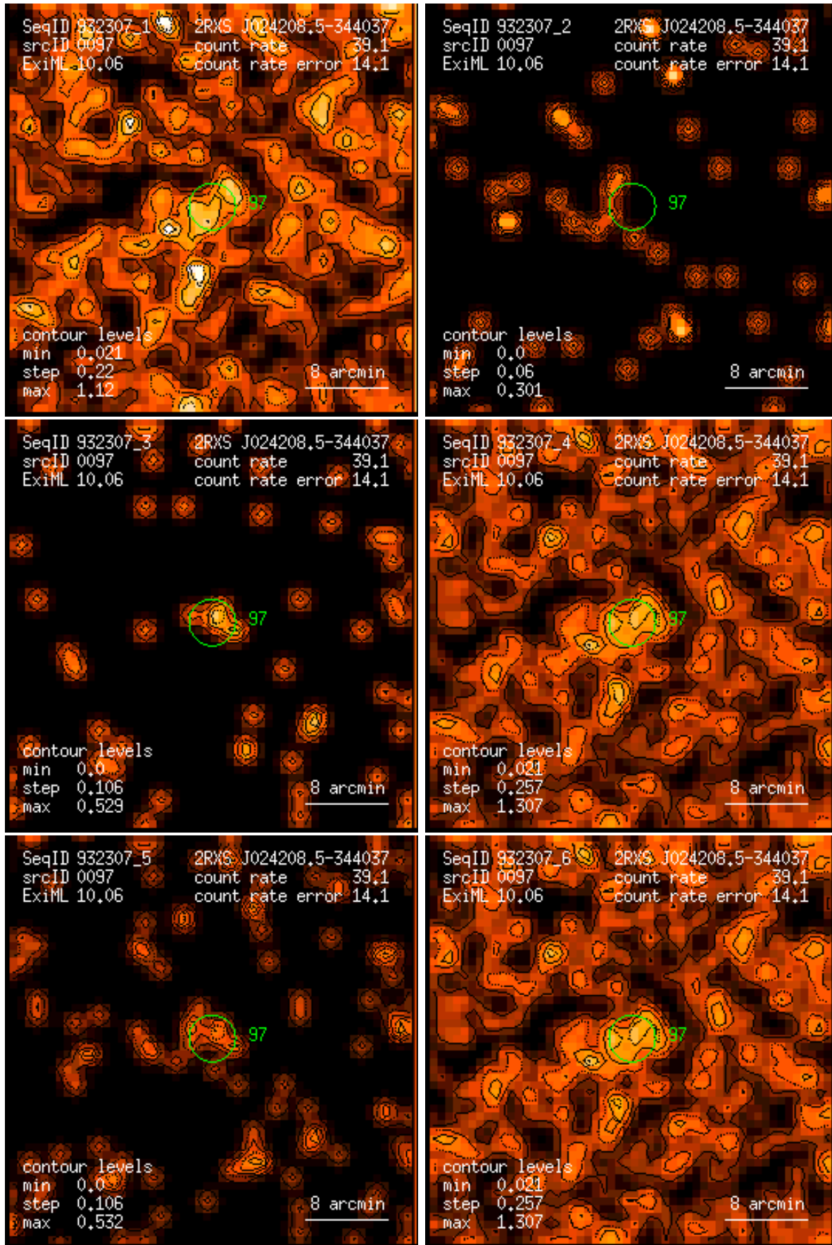
Figure 97: RASS 932307: detection 0097: band rate images, Gaussian filter: (1) PSPC channels 11 – 41, (2) 52 – 90, (3) 91 – 201, (4) 11 – 235, (5) 52 – 201, (6) 11 – 201. Broad band rates in counts/ks. Band rate contour levels in counts/ks/arcmin 2 .
