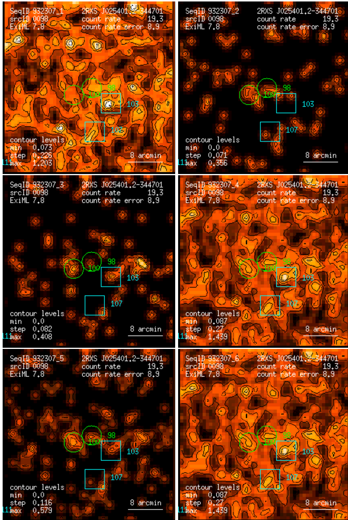
Figure 98: RASS 932307: detection 0098: band rate images, Gaussian filter: (1) PSPC channels 11 – 41, (2) 52 – 90, (3) 91 – 201, (4) 11 – 235, (5) 52 – 201, (6) 11 – 201. Broad band rates in counts/ks. Band rate contour levels in counts/ks/arcmin 2 .
