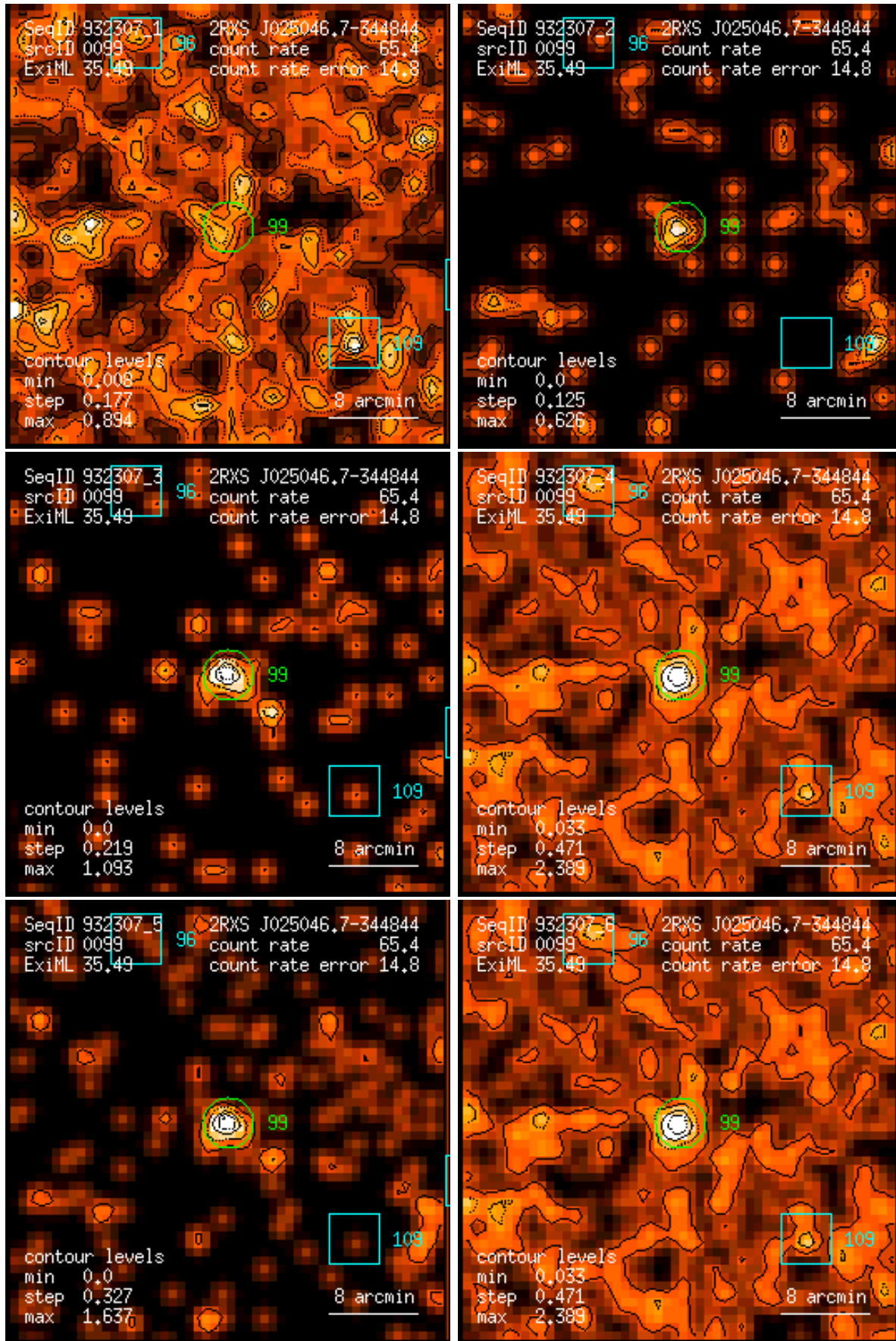
Figure 99: RASS 932307: detection 0099: band rate images, Gaussian filter: (1) PSPC channels 11 – 41, (2) 52 – 90, (3) 91 – 201, (4) 11 – 235, (5) 52 – 201, (6) 11 – 201. Broad band rates in counts/ks. Band rate contour levels in counts/ks/arcmin 2 .
