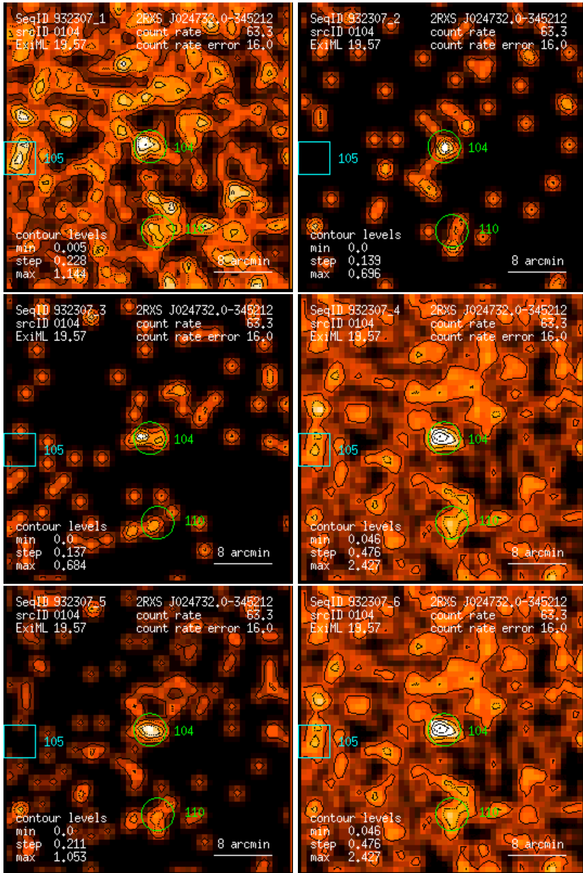
Figure 104: RASS 932307: detection 0104: band rate images, Gaussian filter: (1) PSPC channels 11 – 41, (2) 52 – 90, (3) 91 – 201, (4) 11 – 235, (5) 52 – 201, (6) 11 – 201. Broad band rates in counts/ks. Band rate contour levels in counts/ks/arcmin 2 .
