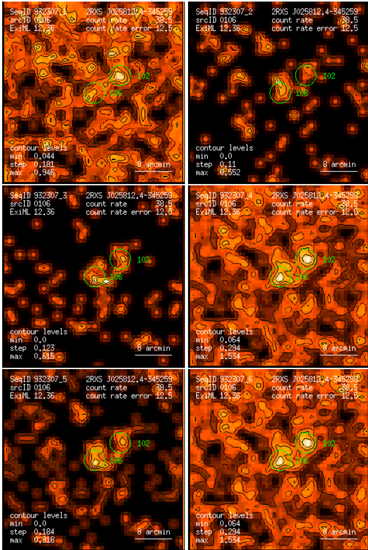
Figure 106: RASS 932307: detection 0106: band rate images, Gaussian filter: (1) PSPC channels 11 – 41, (2) 52 – 90, (3) 91 – 201, (4) 11 – 235, (5) 52 – 201, (6) 11 – 201. Broad band rates in counts/ks. Band rate contour levels in counts/ks/arcmin 2 .
