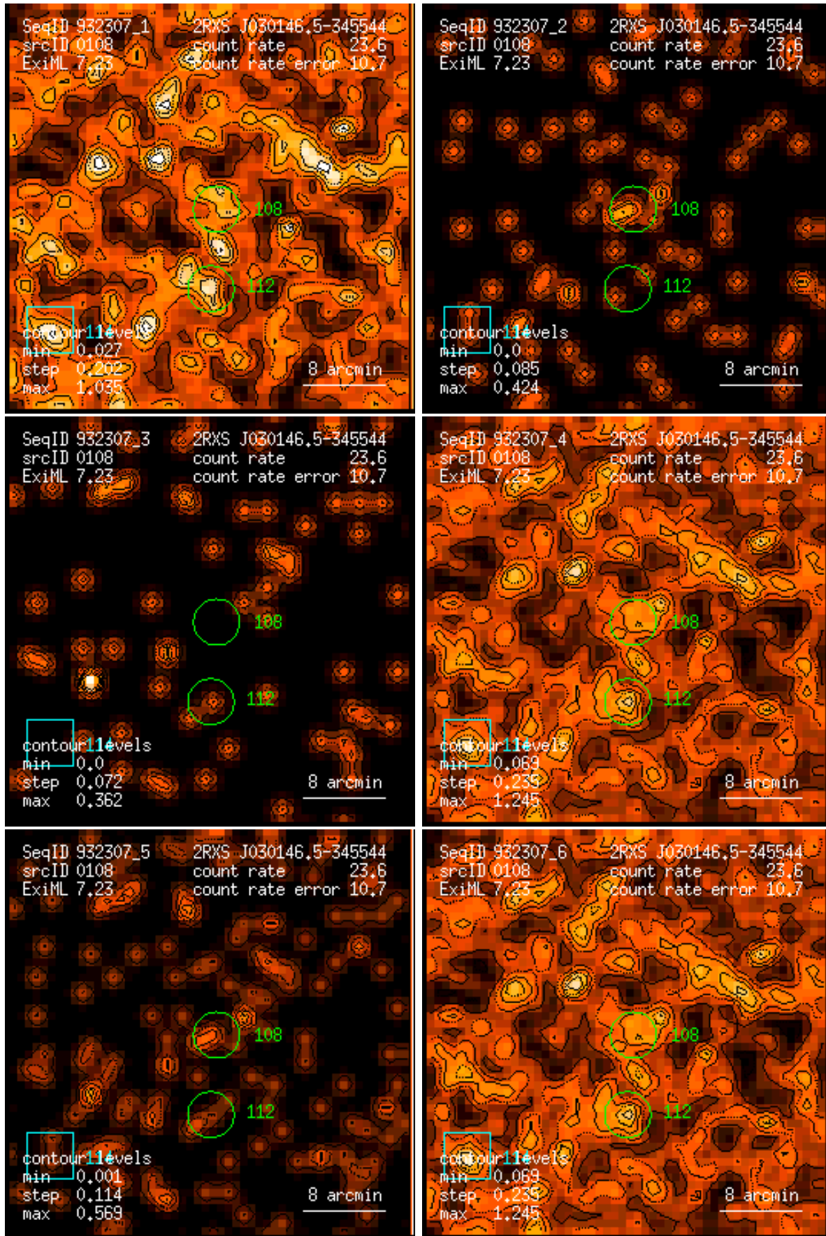
Figure 108: RASS 932307: detection 0108: band rate images, Gaussian filter: (1) PSPC channels 11 – 41, (2) 52 – 90, (3) 91 – 201, (4) 11 – 235, (5) 52 – 201, (6) 11 – 201. Broad band rates in counts/ks. Band rate contour levels in counts/ks/arcmin 2 .
