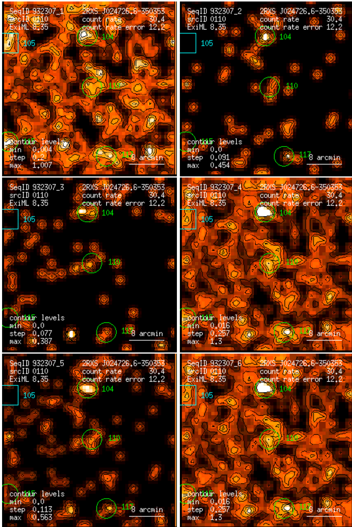
Figure 110: RASS 932307: detection 0110: band rate images, Gaussian filter: (1) PSPC channels 11 – 41, (2) 52 – 90, (3) 91 – 201, (4) 11 – 235, (5) 52 – 201, (6) 11 – 201. Broad band rates in counts/ks. Band rate contour levels in counts/ks/arcmin 2 .
