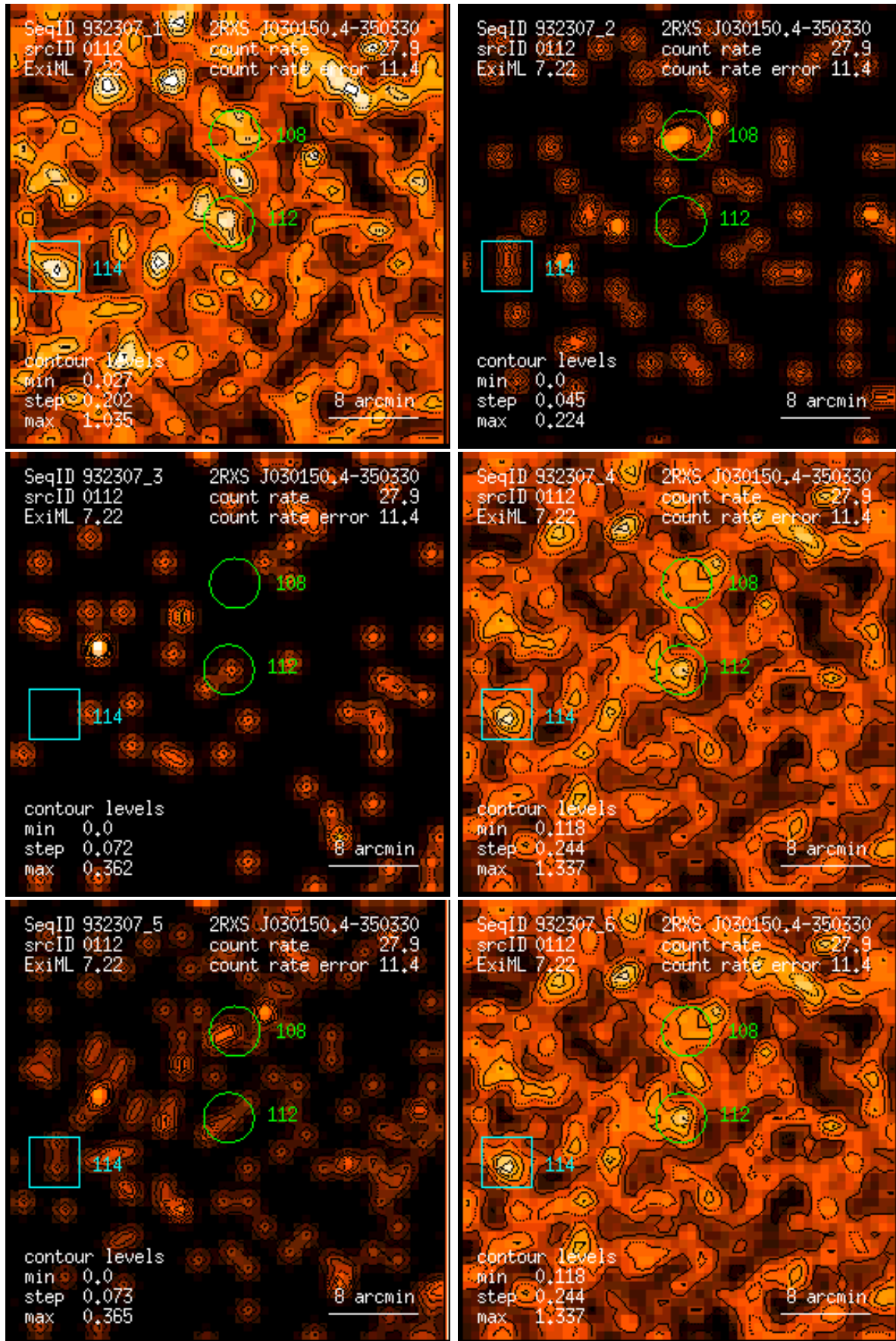
Figure 112: RASS 932307: detection 0112: band rate images, Gaussian filter: (1) PSPC channels 11 – 41, (2) 52 – 90, (3) 91 – 201, (4) 11 – 235, (5) 52 – 201, (6) 11 – 201. Broad band rates in counts/ks. Band rate contour levels in counts/ks/arcmin 2 .
