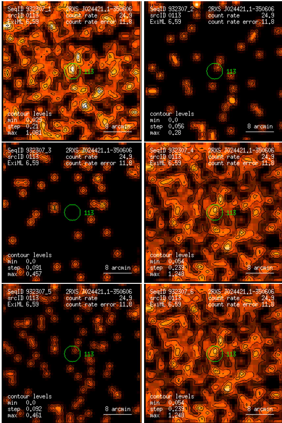
Figure 113: RASS 932307: detection 0113: band rate images, Gaussian filter: (1) PSPC channels 11 – 41, (2) 52 – 90, (3) 91 – 201, (4) 11 – 235, (5) 52 – 201, (6) 11 – 201. Broad band rates in counts/ks. Band rate contour levels in counts/ks/arcmin 2 .
