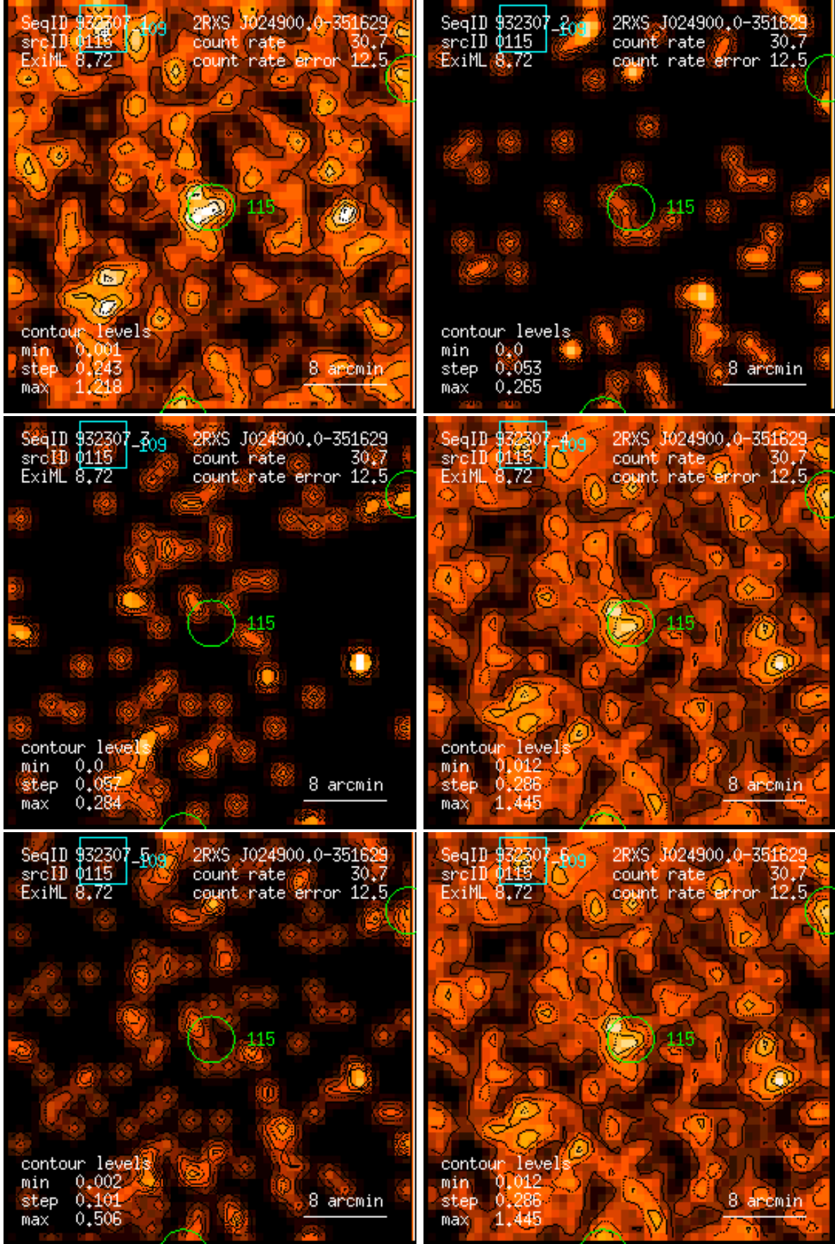
Figure 115: RASS 932307: detection 0115: band rate images, Gaussian filter: (1) PSPC channels 11 – 41, (2) 52 – 90, (3) 91 – 201, (4) 11 – 235, (5) 52 – 201, (6) 11 – 201. Broad band rates in counts/ks. Band rate contour levels in counts/ks/arcmin 2 .
