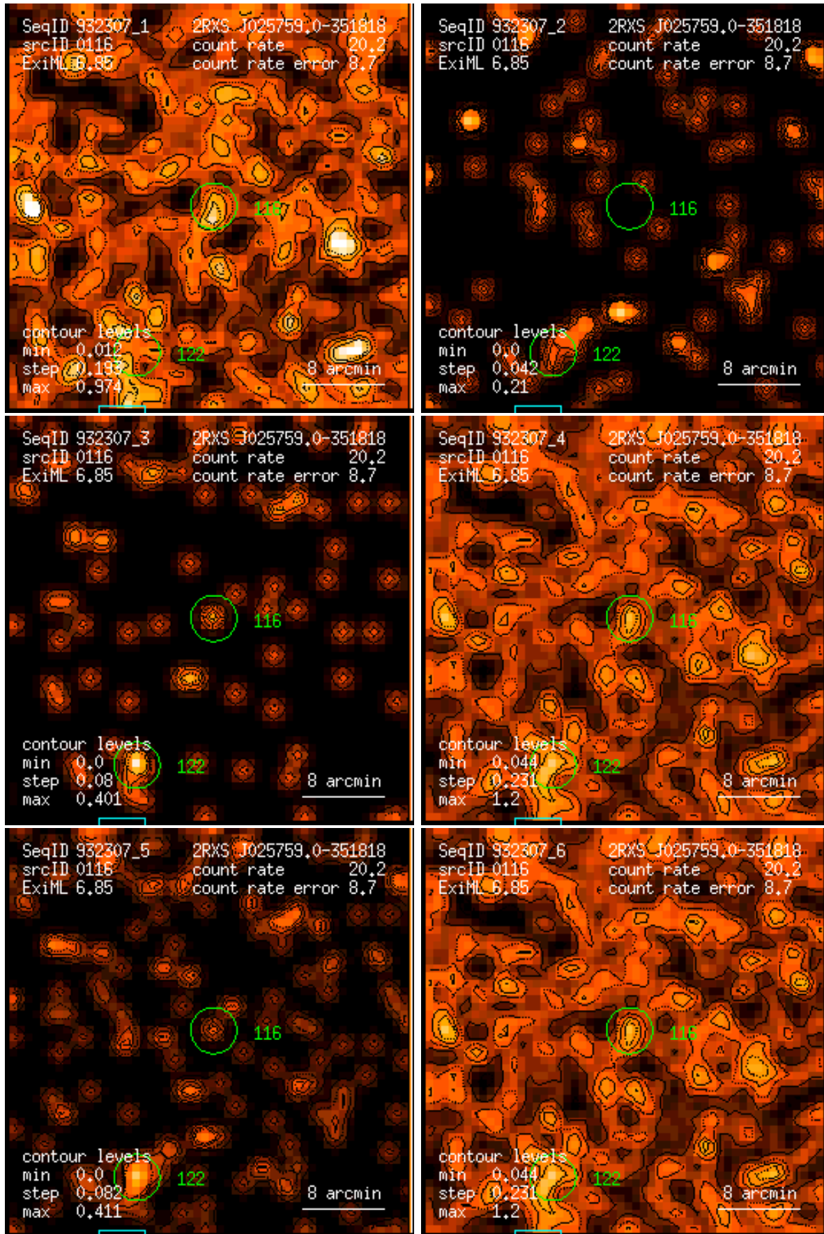
Figure 116: RASS 932307: detection 0116: band rate images, Gaussian filter: (1) PSPC channels 11 – 41, (2) 52 – 90, (3) 91 – 201, (4) 11 – 235, (5) 52 – 201, (6) 11 – 201. Broad band rates in counts/ks. Band rate contour levels in counts/ks/arcmin 2 .
