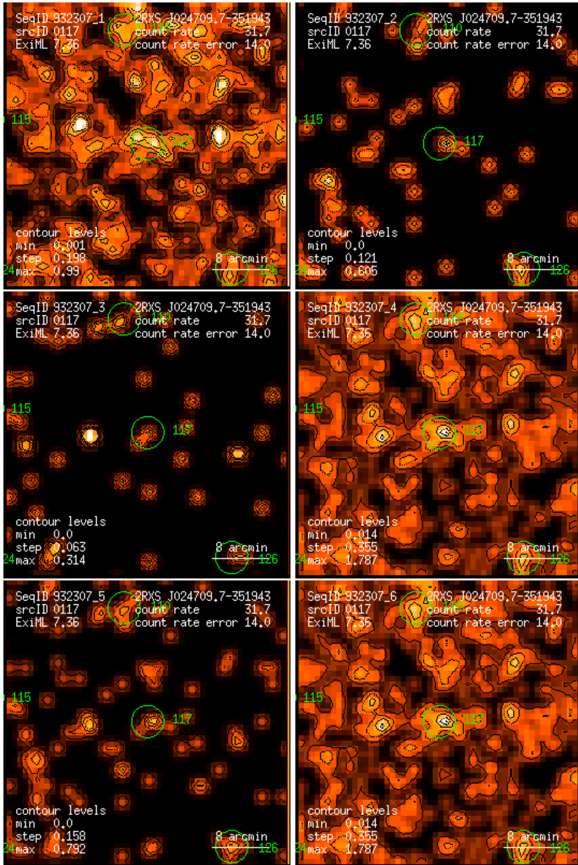
Figure 117: RASS 932307: detection 0117: band rate images, Gaussian filter: (1) PSPPC channels 11 – 41, (2) 52 – 90, (3) 91 – 201, (4) 11 – 235, (5) 52 – 201, (6) 11 – 201. Broad band rates in counts/ks. Band rate contour levels in counts/ks/arcmin 2 .
