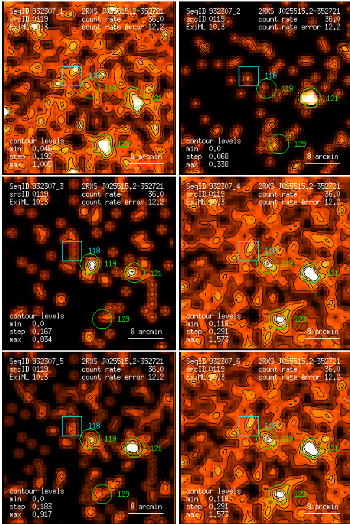
Figure 119: RASS 932307: detection 0119: band rate images, Gaussian filter: (1) PSPC channels 11 – 41, (2) 52 – 90, (3) 91 – 201, (4) 11 – 235, (5) 52 – 201, (6) 11 – 201. Broad band rates in counts/ks. Band rate contour levels in counts/ks/arcmin 2 .
