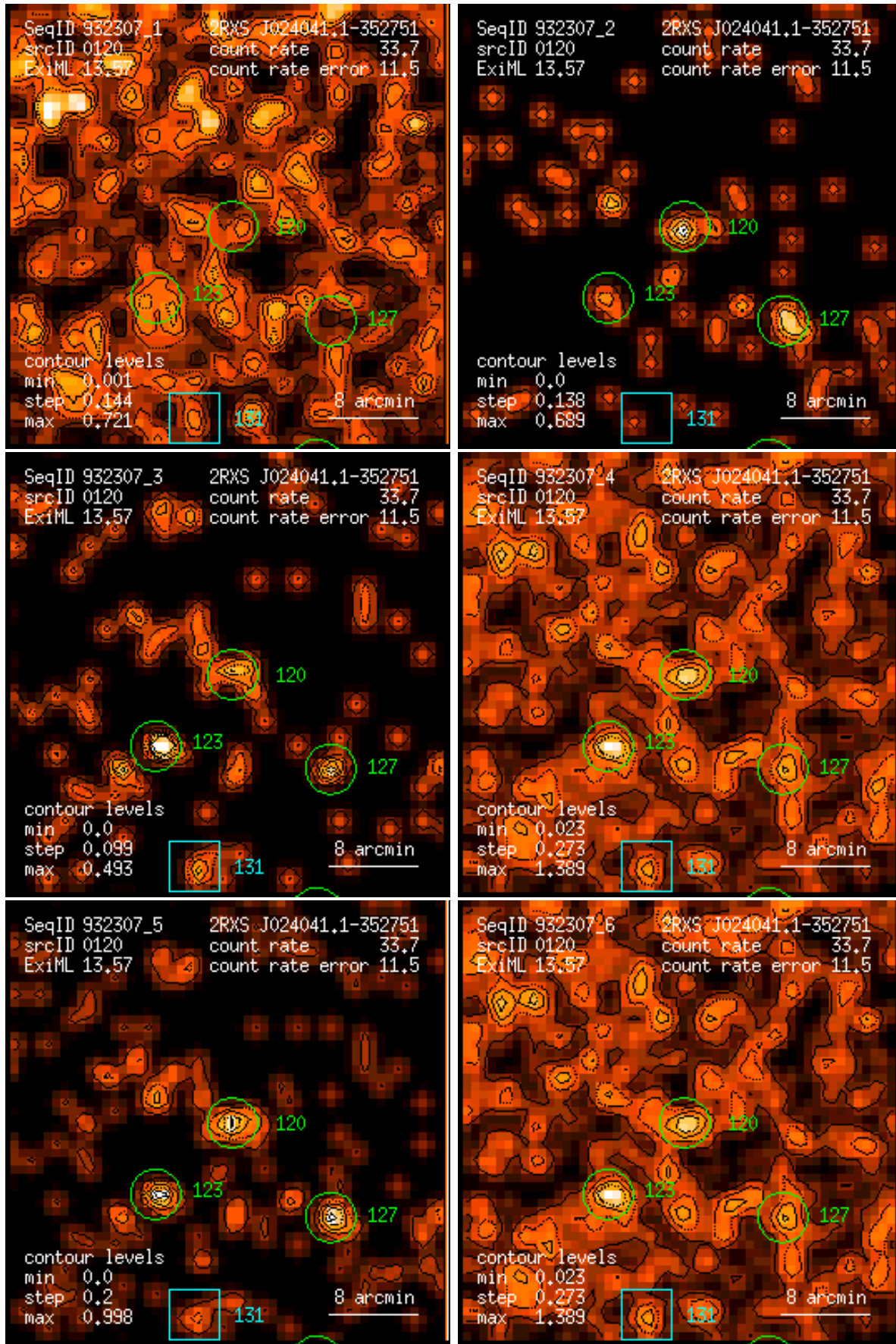
Figure 120: RASS 932307: detection 0120: band rate images, Gaussian filter: (1) PSPC channels 11 – 41, (2) 52 – 90, (3) 91 – 201, (4) 11 – 235, (5) 52 – 201, (6) 11 – 201. Broad band rates in counts/ks. Band rate contour levels in counts/ks/arcmin 2 .
