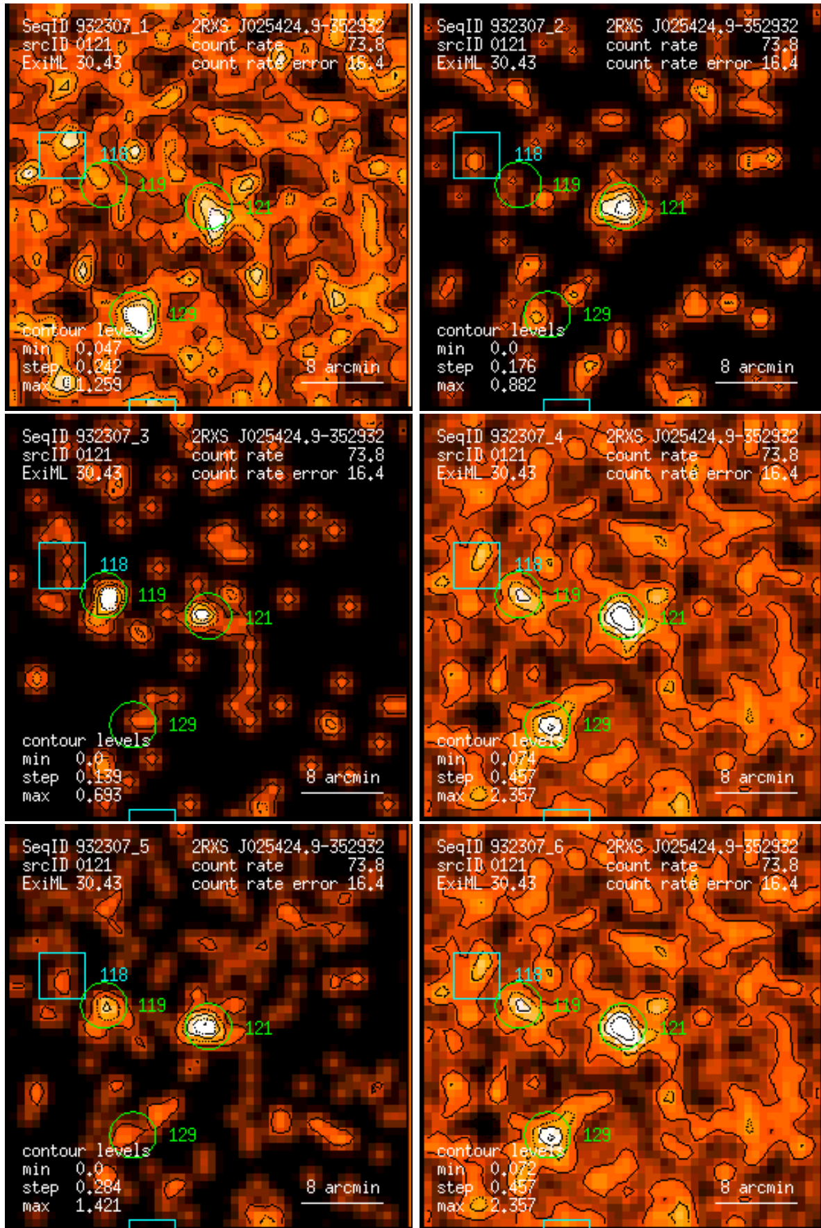
Figure 121: RASS 932307: detection 0121: band rate images, Gaussian filter: (1) PSPC channels 11 – 41, (2) 52 – 90, (3) 91 – 201, (4) 11 – 235, (5) 52 – 201, (6) 11 – 201. Broad band rates in counts/ks. Band rate contour levels in counts/ks/arcmin 2 .
