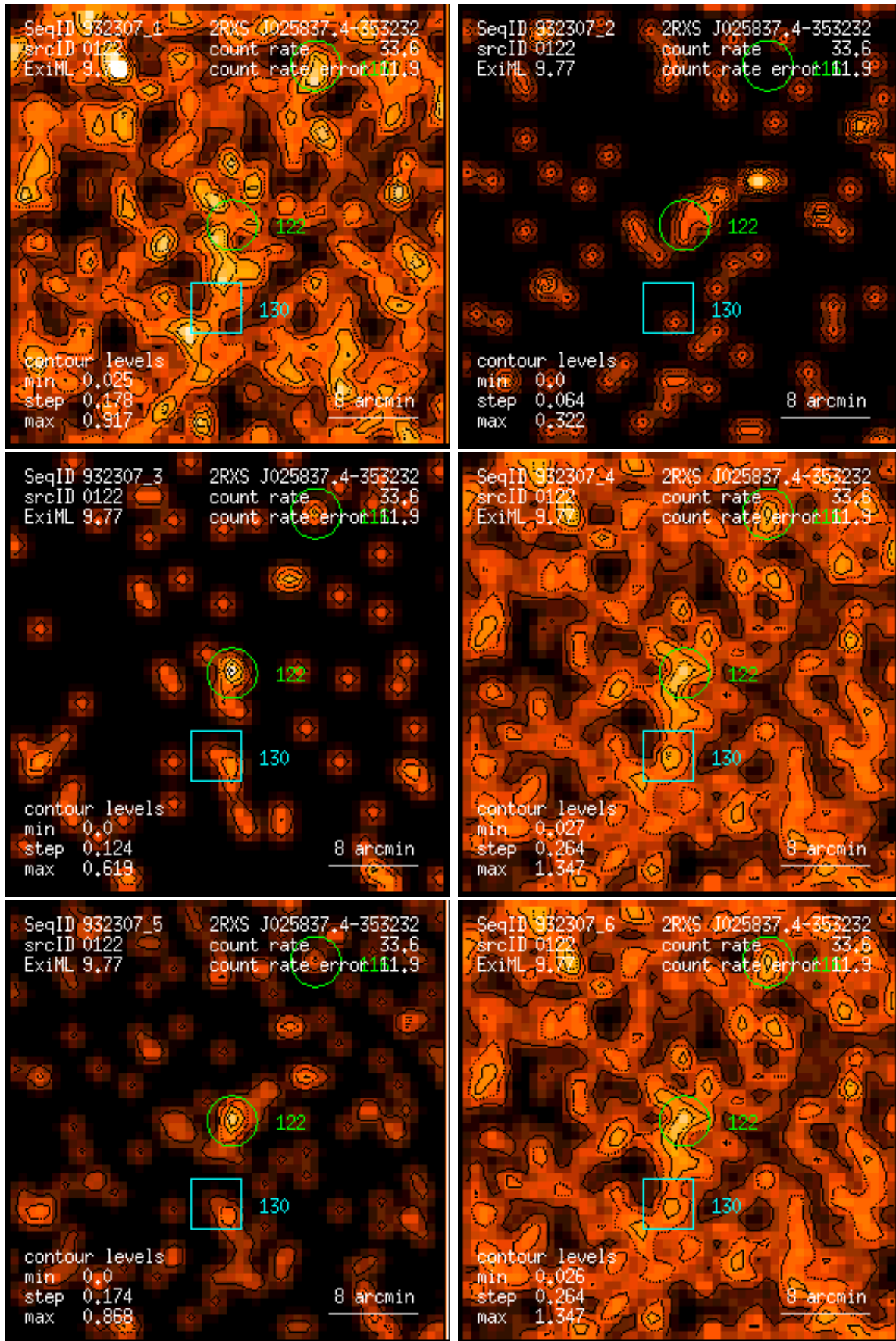
Figure 122: RASS 932307: detection 0122: band rate images, Gaussian filter: (1) PSPC channels 11 – 41, (2) 52 – 90, (3) 91 – 201, (4) 11 – 235, (5) 52 – 201, (6) 11 – 201. Broad band rates in counts/ks. Band rate contour levels in counts/ks/arcmin 2 .
