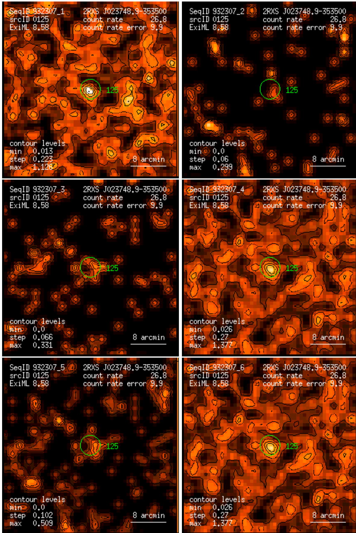
Figure 125: RASS 932307: detection 0125: band rate images, Gaussian filter: (1) PSPC channels 11 – 41, (2) 52 – 90, (3) 91 – 201, (4) 11 – 235, (5) 52 – 201, (6) 11 – 201. Broad band rates in counts/ks. Band rate contour levels in counts/ks/arcmin 2 .
