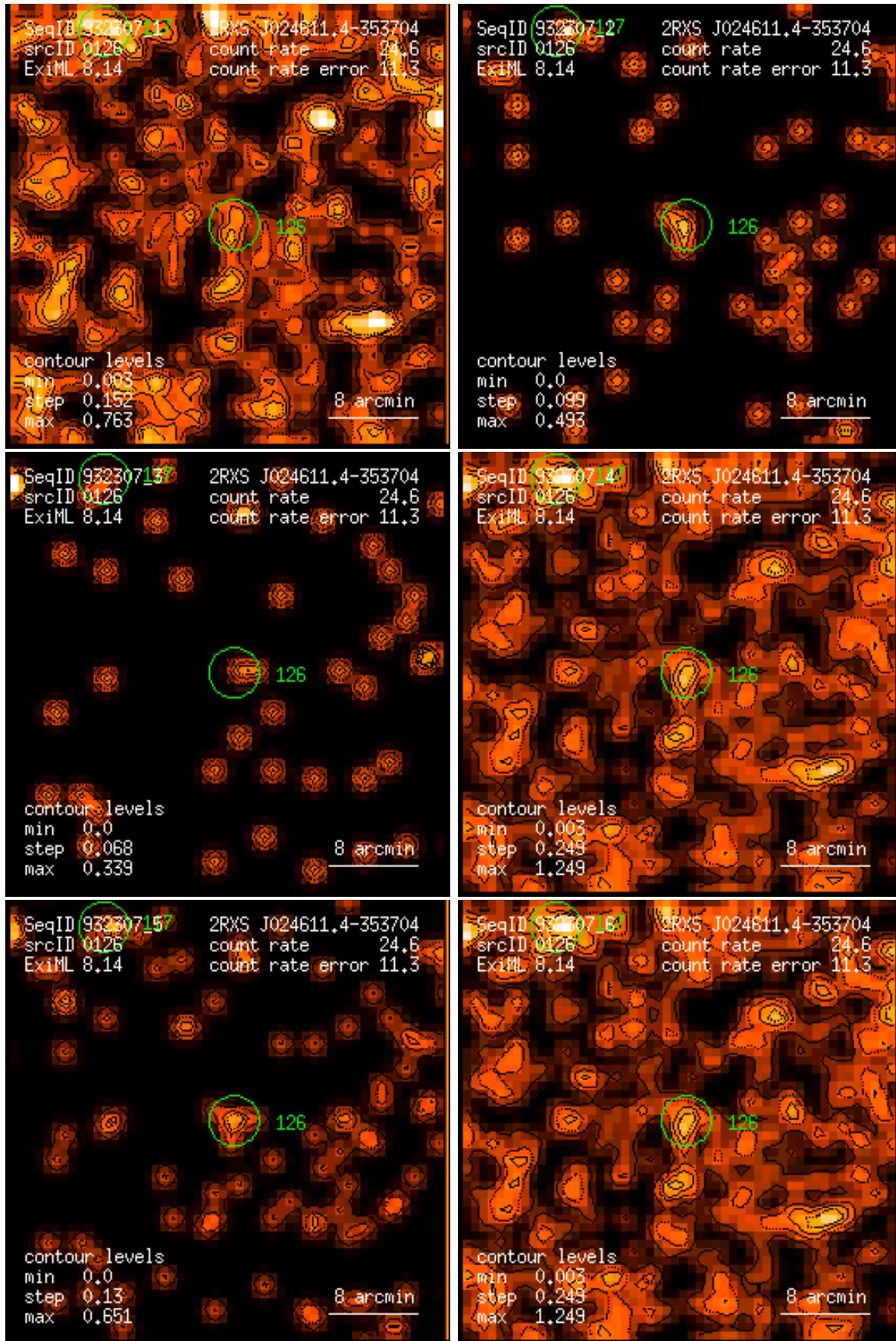
Figure 126: RASS 932307: detection 0126: band rate images, Gaussian filter: (1) PSPC channels 11 – 41, (2) 52 – 90, (3) 91 – 201, (4) 11 – 235, (5) 52 – 201, (6) 11 – 201. Broad band rates in counts/ks. Band rate contour levels in counts/ks/arcmin 2 .
