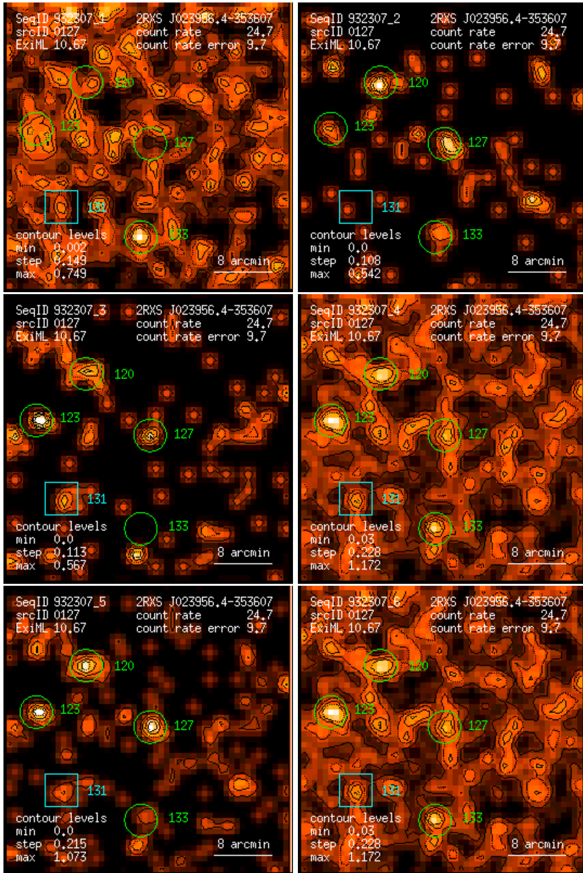
Figure 127: RASS 932307: detection 0127: band rate images, Gaussian filter: (1) PSPC channels 11 – 41, (2) 52 – 90, (3) 91 – 201, (4) 11 – 235, (5) 52 – 201, (6) 11 – 201. Broad band rates in counts/ks. Band rate contour levels in counts/ks/arcmin 2 .
