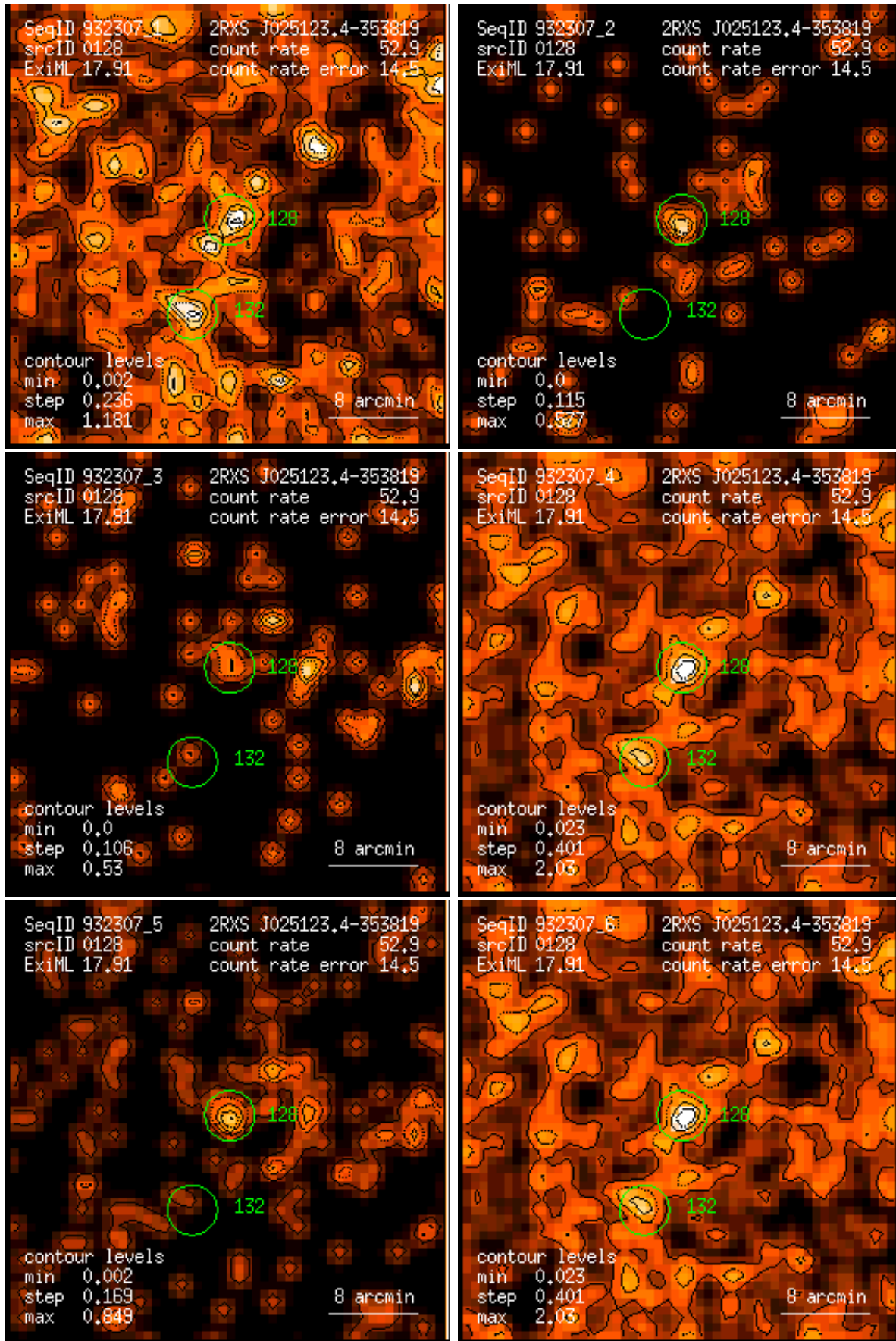
Figure 128: RASS 932307: detection 0128: band rate images, Gaussian filter: (1) PSPC channels 11 – 41, (2) 52 – 90, (3) 91 – 201, (4) 11 – 235, (5) 52 – 201, (6) 11 – 201. Broad band rates in counts/ks. Band rate contour levels in counts/ks/arcmin 2 .
