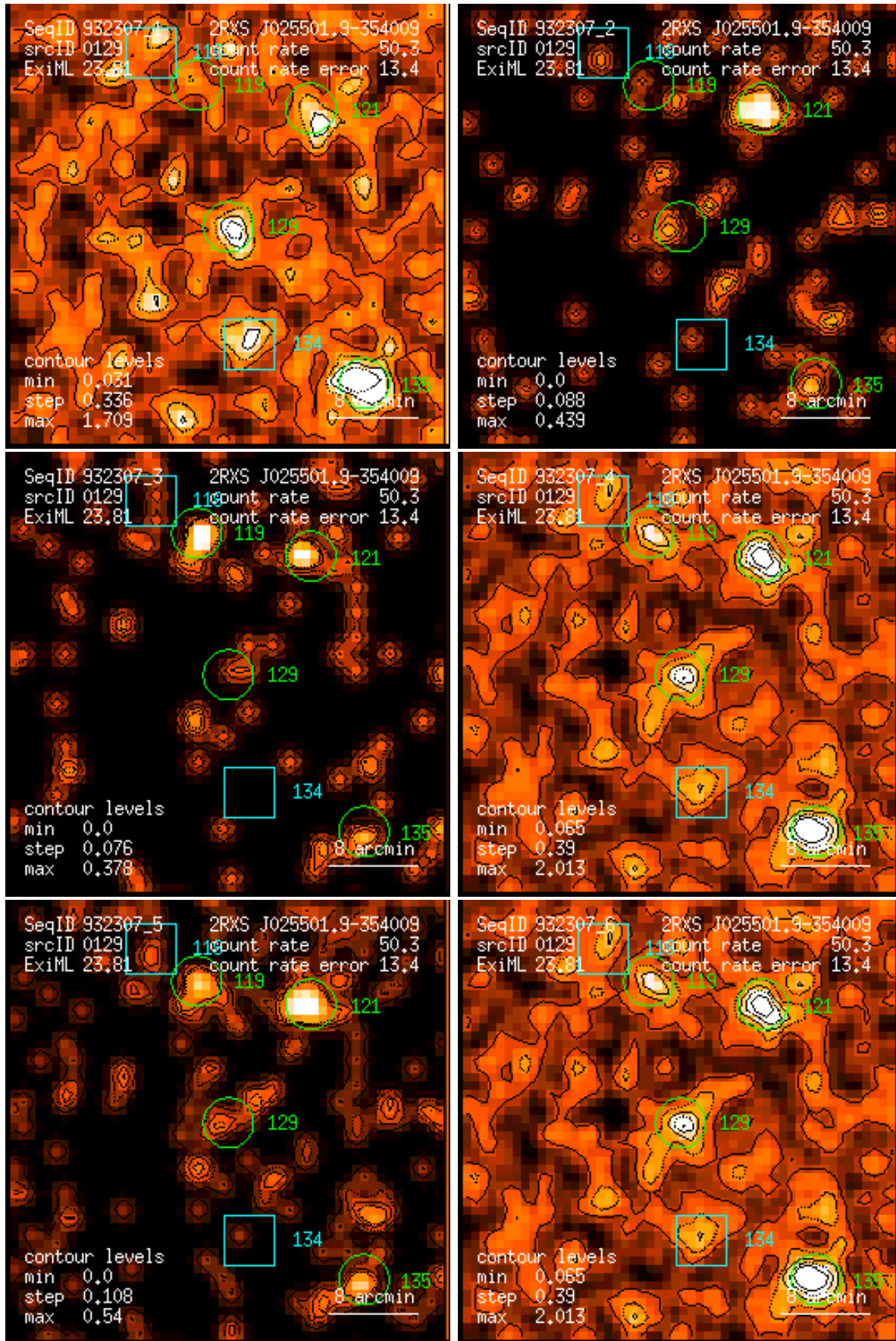
Figure 129: RASS 932307: detection 0129: band rate images, Gaussian filter: (1) PSPC channels 11 – 41, (2) 52 – 90, (3) 91 – 201, (4) 11 – 235, (5) 52 – 201, (6) 11 – 201. Broad band rates in counts/ks. Band rate contour levels in counts/ks/arcmin 2 .
