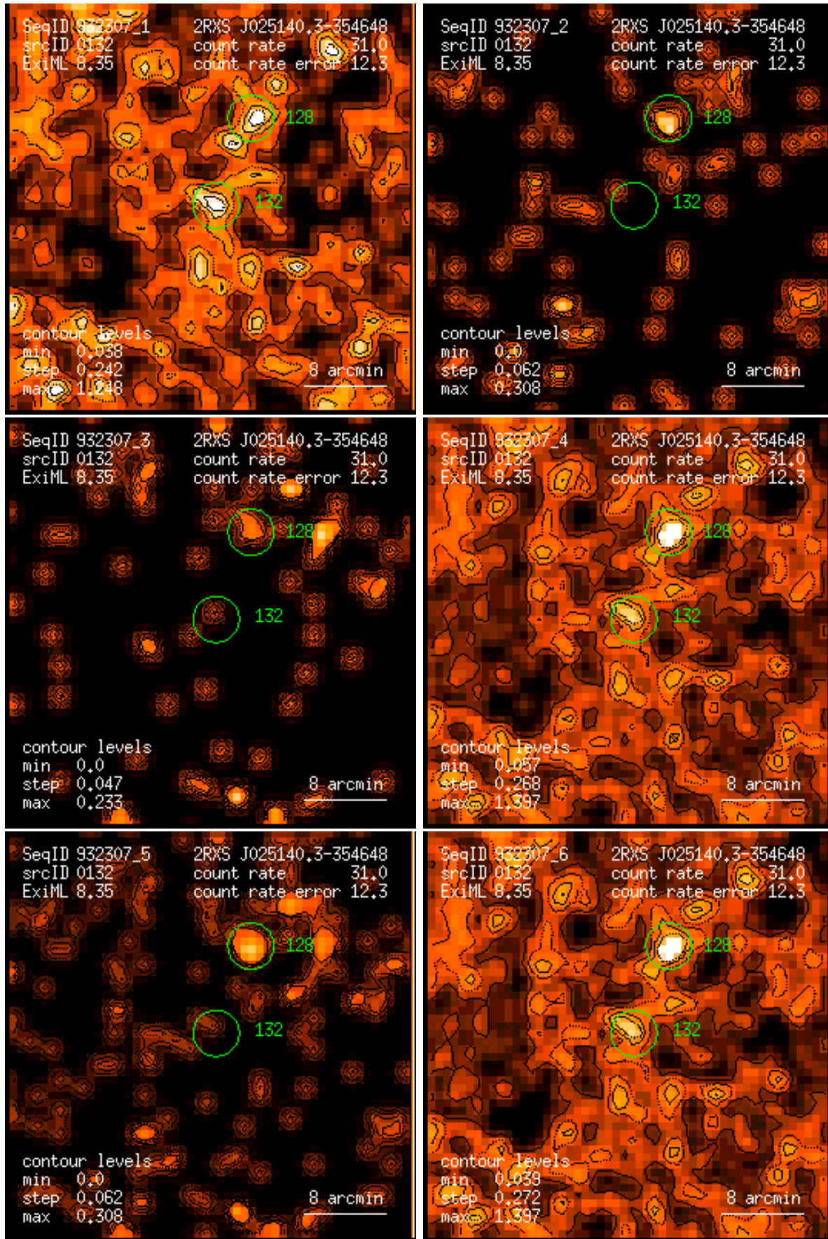
Figure 132: RASS 932307: detection 0132: band rate images, Gaussian filter: (1) PSPC channels 11 – 41, (2) 52 – 90, (3) 91 – 201, (4) 11 – 235, (5) 52 – 201, (6) 11 – 201. Broad band rates in counts/ks. Band rate contour levels in counts/ks/arcmin 2 .
