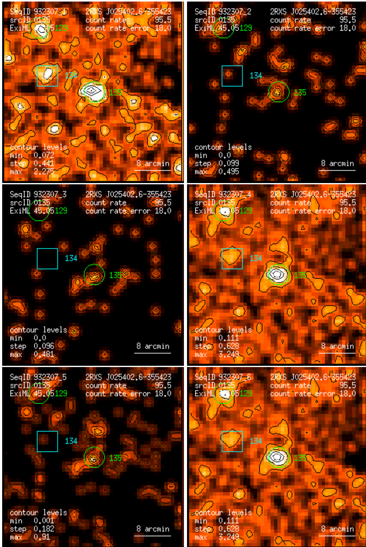
Figure 135: RASS 932307: detection 0135: band rate images, Gaussian filter: (1) PSPC channels 11 – 41, (2) 52 – 90, (3) 91 – 201, (4) 11 – 235, (5) 52 – 201, (6) 11 – 201. Broad band rates in counts/ks. Band rate contour levels in counts/ks/arcmin 2 .
