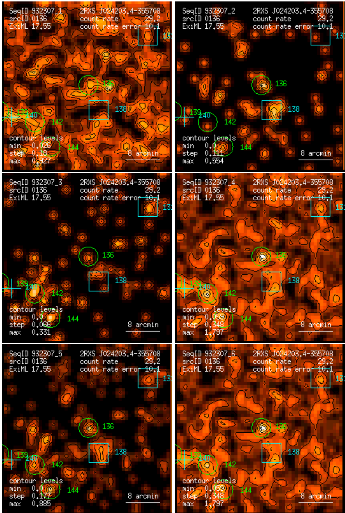
Figure 136: RASS 932307: detection 0136: band rate images, Gaussian filter: (1) PSPC channels 11 – 41, (2) 52 – 90, (3) 91 – 201, (4) 11 – 235, (5) 52 – 201, (6) 11 – 201. Broad band rates in counts/ks. Band rate contour levels in counts/ks/arcmin 2 .
