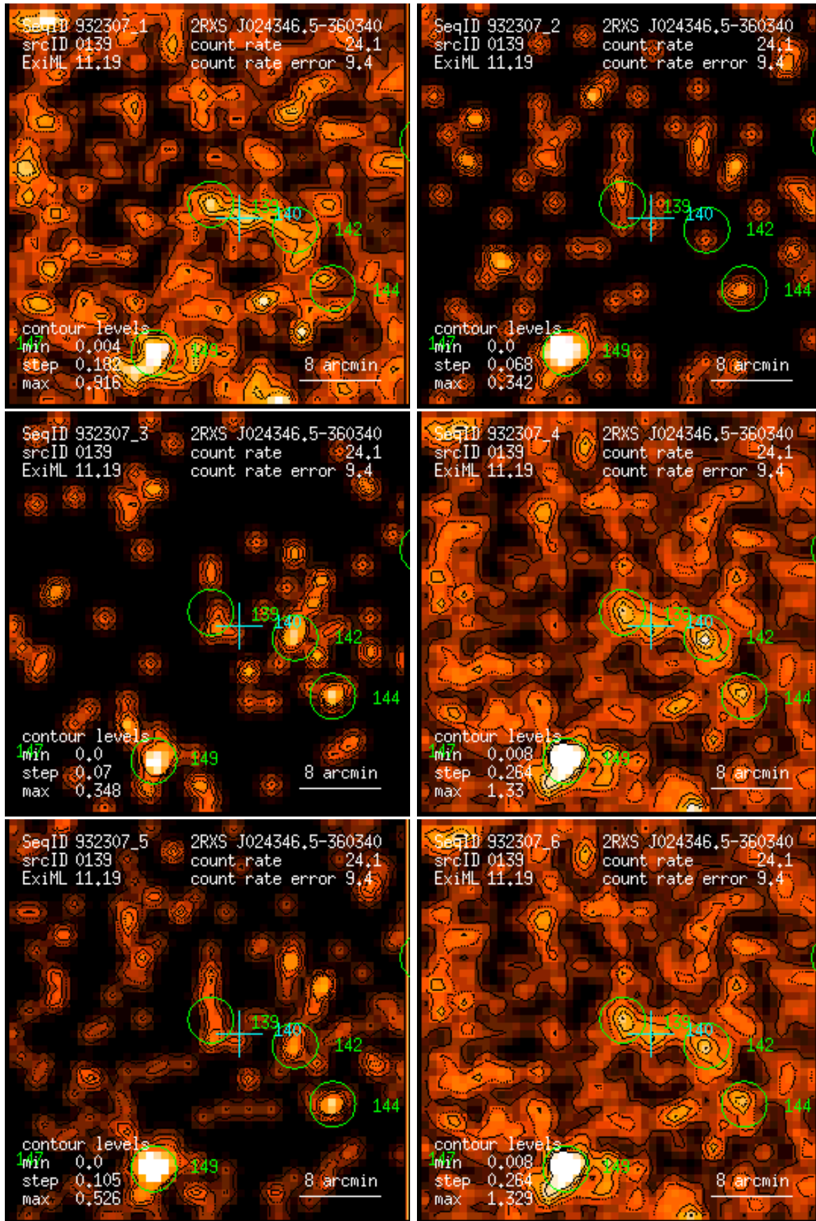
Figure 139: RASS 932307: detection 0139: band rate images, Gaussian filter: (1) PSPC channels 11 – 41, (2) 52 – 90, (3) 91 – 201, (4) 11 – 235, (5) 52 – 201, (6) 11 – 201. Broad band rates in counts/ks. Band rate contour levels in counts/ks/arcmin 2 .
