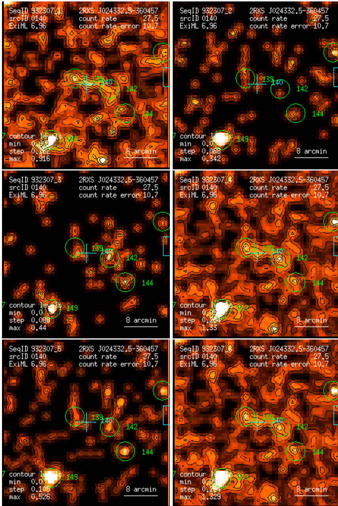
Figure 140: RASS 932307: detection 0140: band rate images, Gaussian filter: (1) PSPC channels 11 – 41, (2) 52 – 90, (3) 91 – 201, (4) 11 – 235, (5) 52 – 201, (6) 11 – 201. Broad band rates in counts/ks. Band rate contour levels in counts/ks/arcmin 2 .
