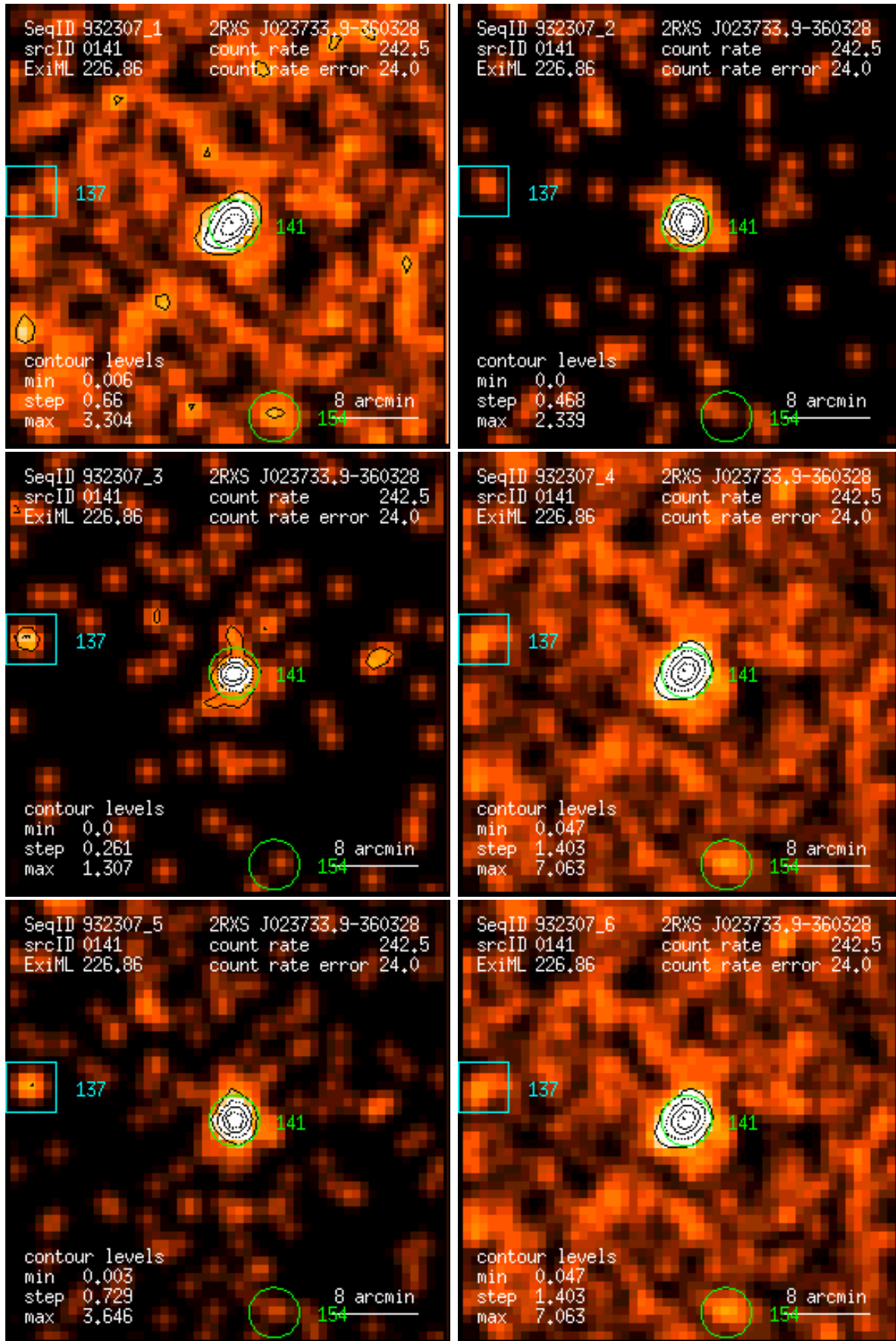
Figure 141: RASS 932307: detection 0141: band rate images, Gaussian filter: (1) PSPC channels 11 – 41, (2) 52 – 90, (3) 91 – 201, (4) 11 – 235, (5) 52 – 201, (6) 11 – 201. Broad band rates in counts/ks. Band rate contour levels in counts/ks/arcmin 2 .
