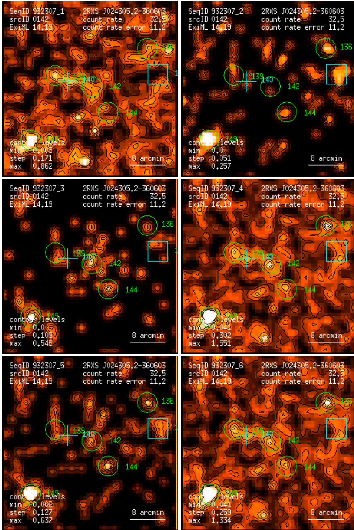
Figure 142: RASS 932307: detection 0142: band rate images, Gaussian filter: (1) PSPC channels 11 – 41, (2) 52 – 90, (3) 91 – 201, (4) 11 – 235, (5) 52 – 201, (6) 11 – 201. Broad band rates in counts/ks. Band rate contour levels in counts/ks/arcmin 2 .
