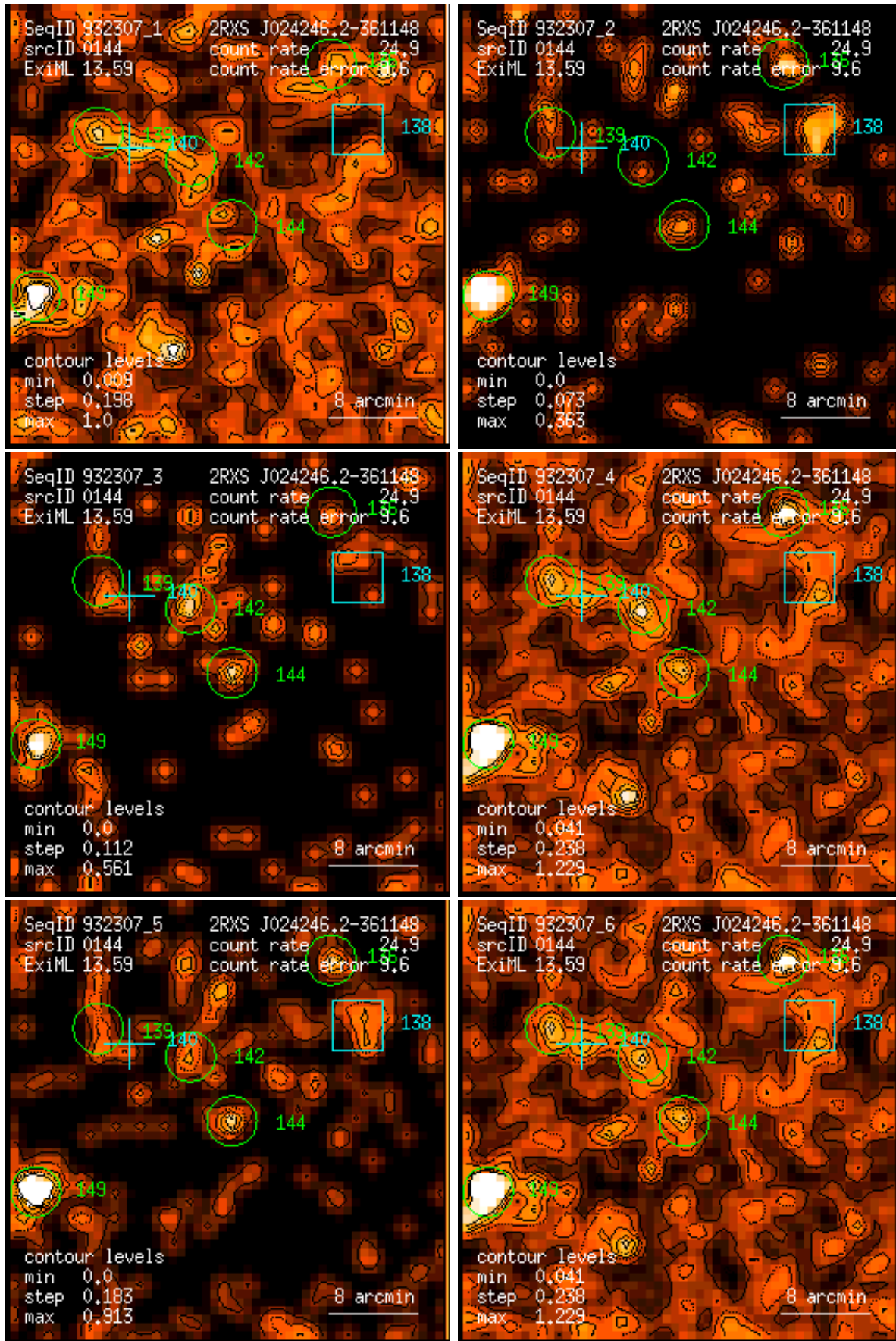
Figure 144: RASS 932307: detection 0144: band rate images, Gaussian filter: (1) PSPC channels 11 – 41, (2) 52 – 90, (3) 91 – 201, (4) 11 – 235, (5) 52 – 201, (6) 11 – 201. Broad band rates in counts/ks. Band rate contour levels in counts/ks/arcmin 2 .
