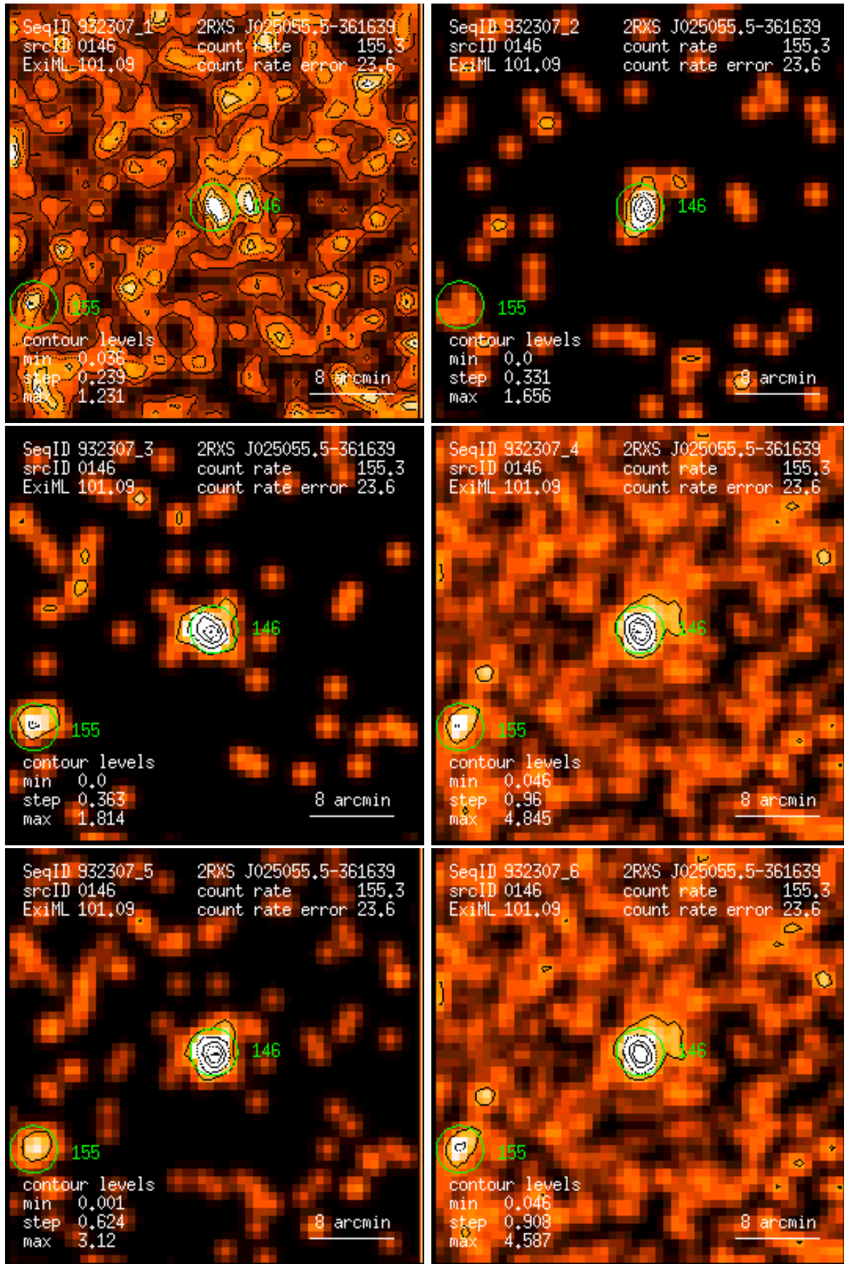
Figure 146: RASS 932307: detection 0146: band rate images, Gaussian filter: (1) PSPC channels 11 – 41, (2) 52 – 90, (3) 91 – 201, (4) 11 – 235, (5) 52 – 201, (6) 11 – 201. Broad band rates in counts/ks. Band rate contour levels in counts/ks/arcmin 2 .
