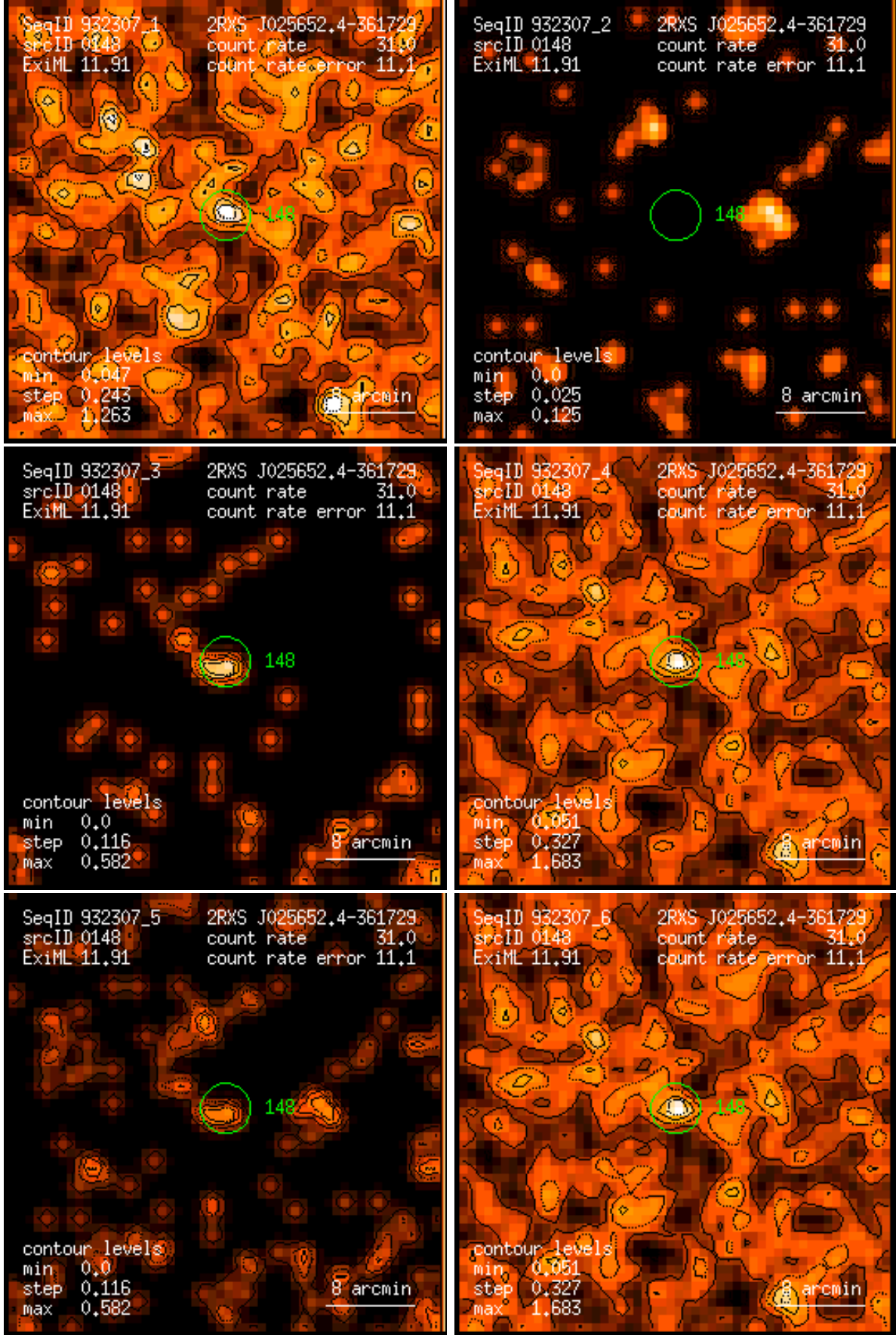
Figure 148: RASS 932307: detection 0148: band rate images, Gaussian filter: (1) PSPC channels 11 – 41, (2) 52 – 90, (3) 91 – 201, (4) 11 – 235, (5) 52 – 201, (6) 11 – 201. Broad band rates in counts/ks. Band rate contour levels in counts/ks/arcmin 2 .
