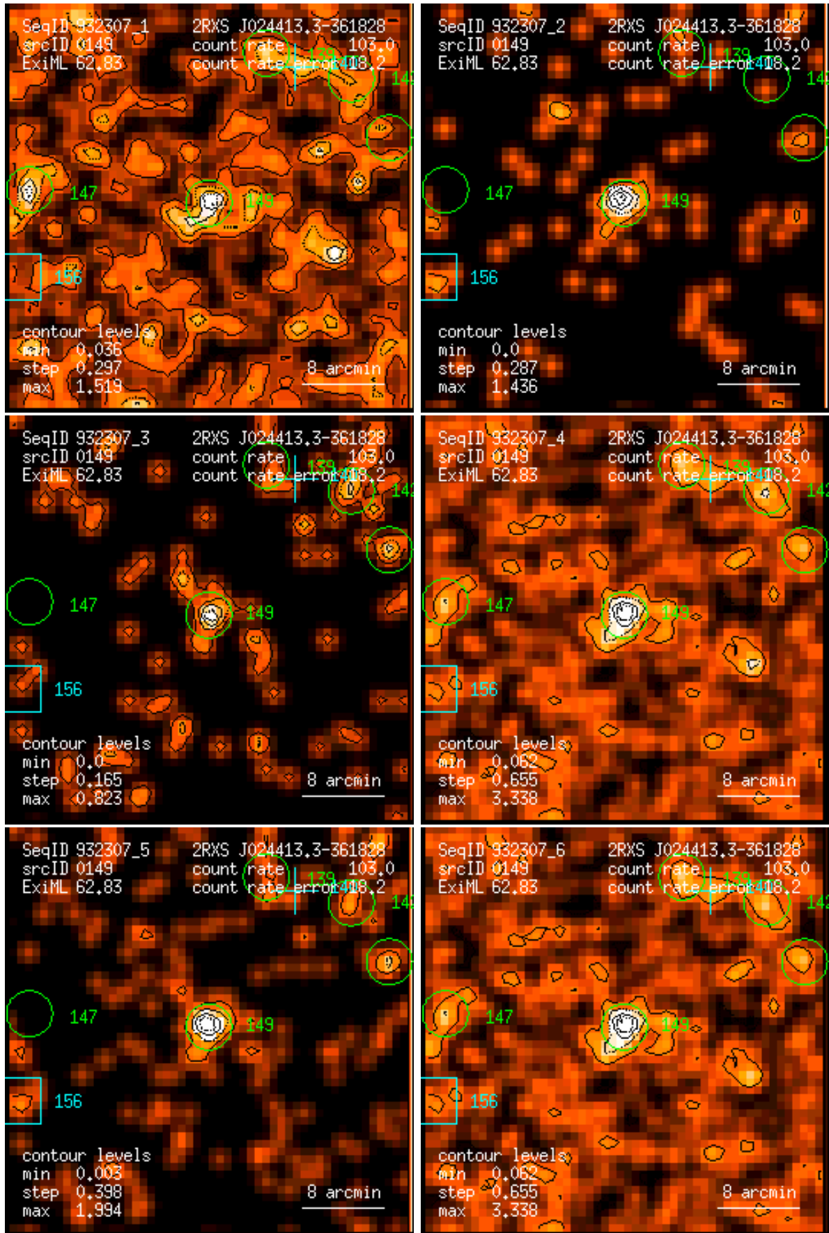
Figure 149: RASS 932307: detection 0149: band rate images, Gaussian filter: (1) PSPC channels 11 – 41, (2) 52 – 90, (3) 91 – 201, (4) 11 – 235, (5) 52 – 201, (6) 11 – 201. Broad band rates in counts/ks. Band rate contour levels in counts/ks/arcmin 2 .
