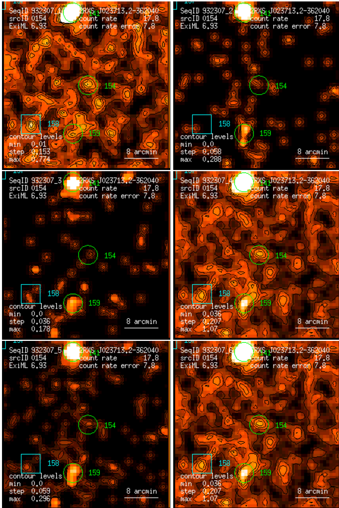
Figure 154: RASS 932307: detection 0154: band rate images, Gaussian filter: (1) PSPC channels 11 – 41, (2) 52 – 90, (3) 91 – 201, (4) 11 – 235, (5) 52 – 201, (6) 11 – 201. Broad band rates in counts/ks. Band rate contour levels in counts/ks/arcmin 2 .
